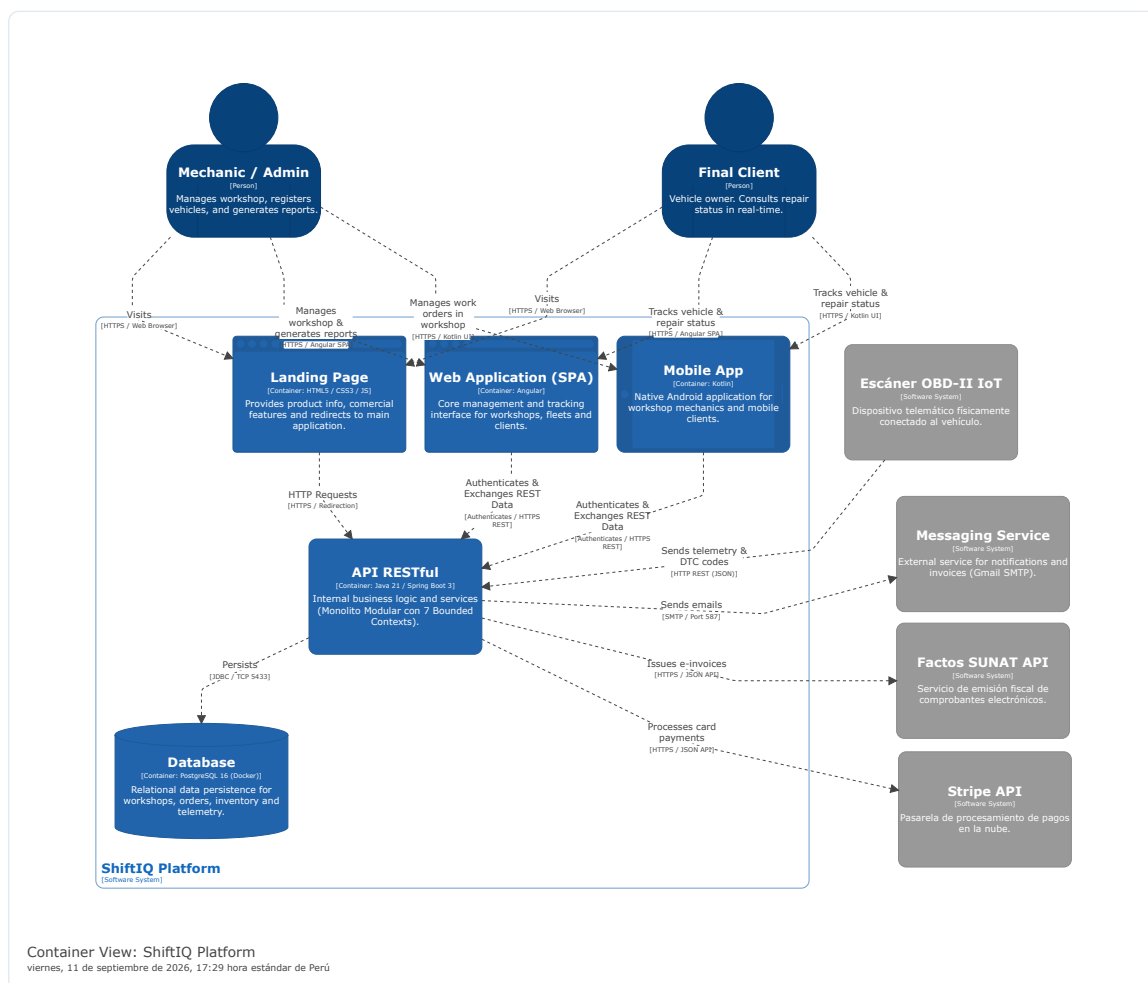
Figura 32: Diagrama de Contenedores – ShiftIQ Platform.
