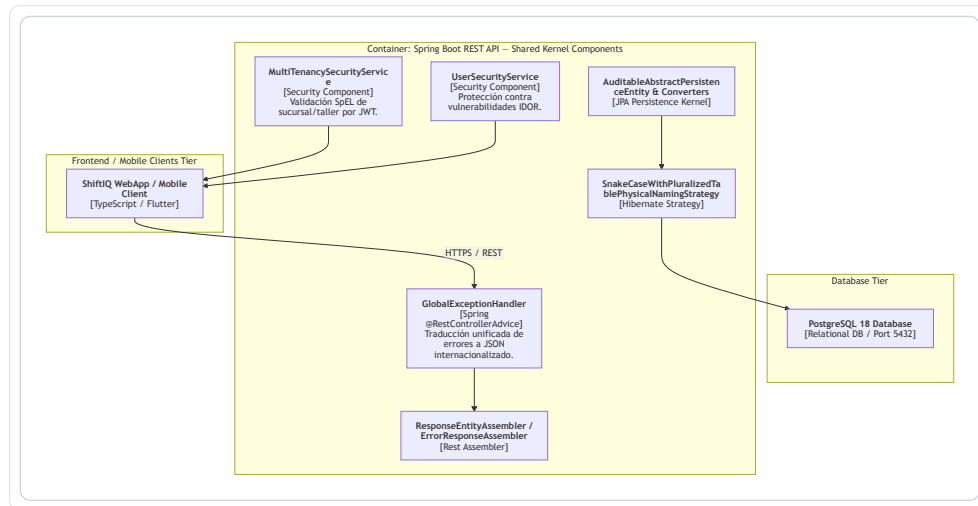
Figura 38: Component Diagram (C4 Level 3) – Shared Kernel
