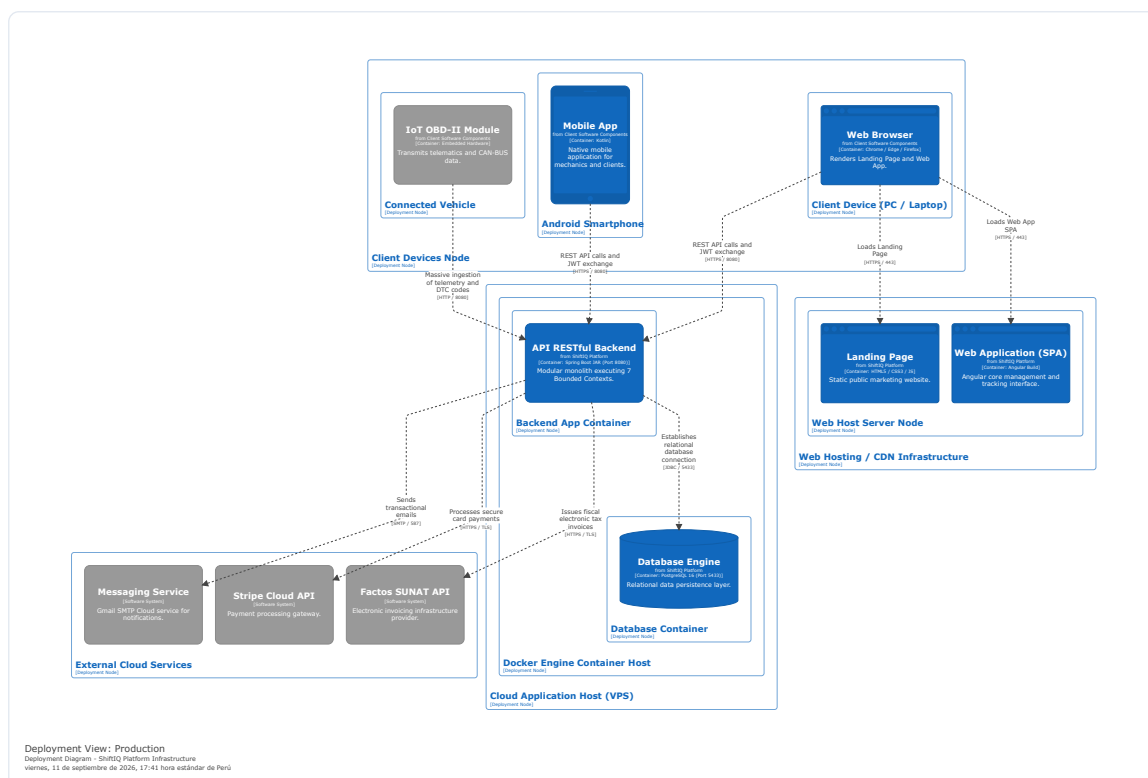
Figura 33: Diagrama de Despliegue – ShiftIQ Platform Infrastructure.
