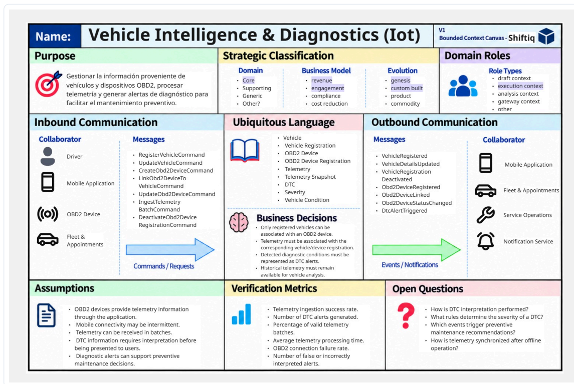
Figura 26: Bounded Context Canvas – Vehicle Intelligence &amp; Diagnostics.
