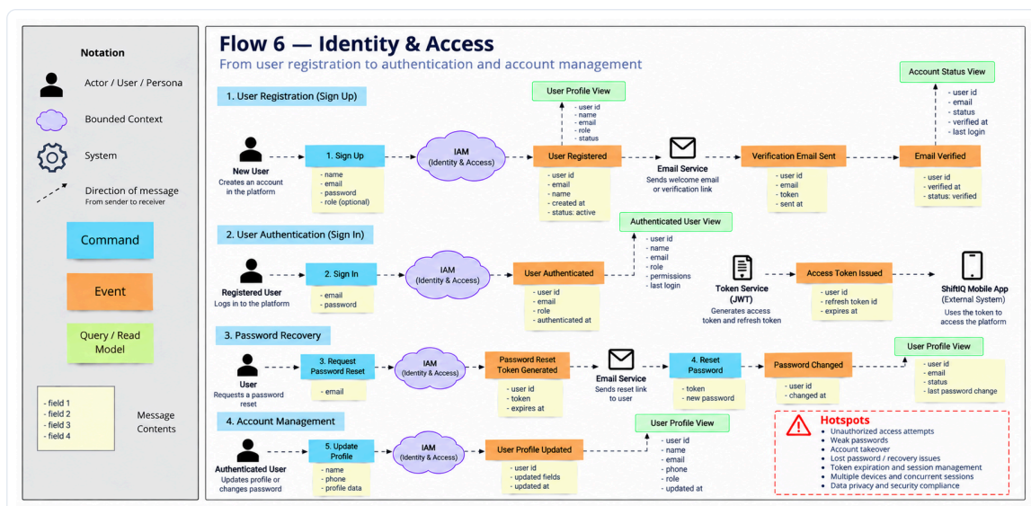
Figura 22: Domain Message Flow – Identity &amp; Access.
