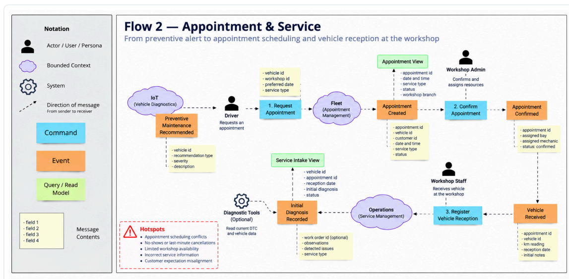
Figura 18: Domain Message Flow – Appointment & Service.
