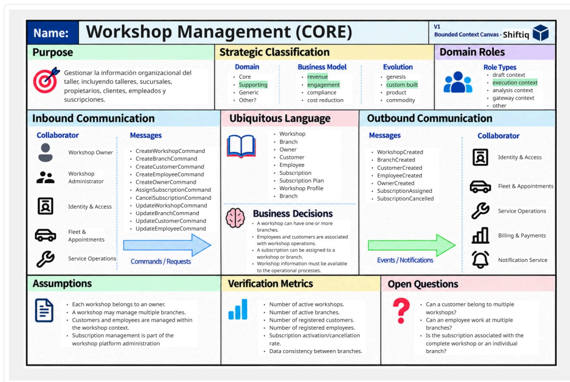
Figura 24: Bounded Context Canvas – Workshop Management.
