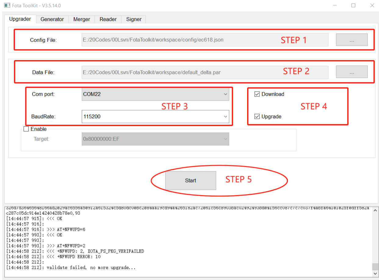
Figure 3-7. GUI for Dowloading An Upgrade File via AT Command
