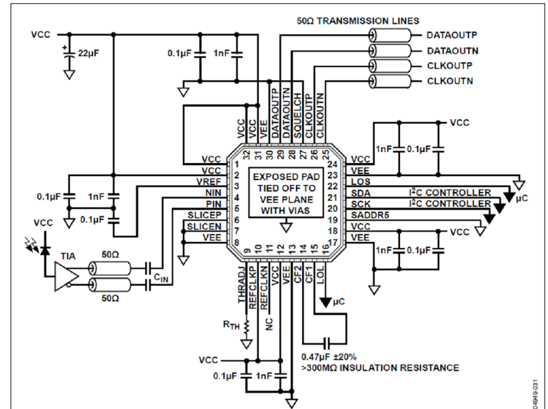
Figure 24. Typical ADN2814 Applications Circuit
