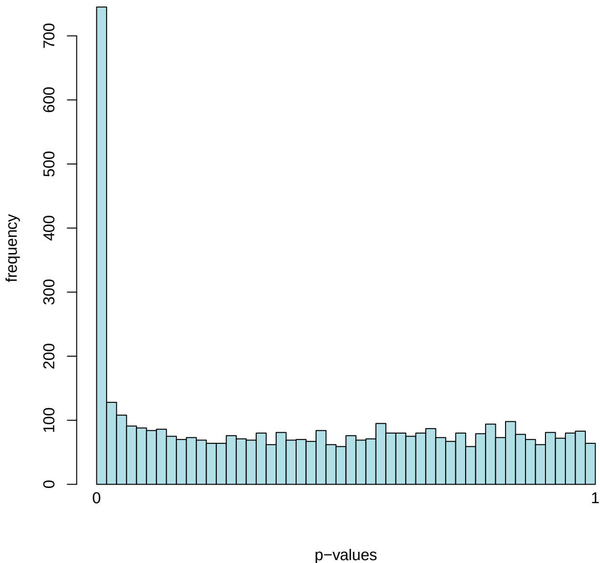
Histogram of p-values for Genomic_Background: Mutant vs WildType
