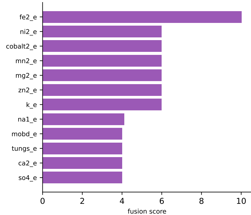
(c) iAF1260, targeted trace-metal sweep (12 of 15 candidates shown)
