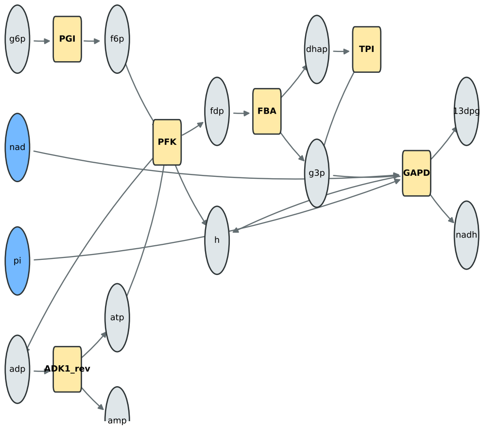
(a) Illustrative reaction network (6 real E. coli reactions: PGI, ADK1, PFK, FBA, TPI, GAPD)
