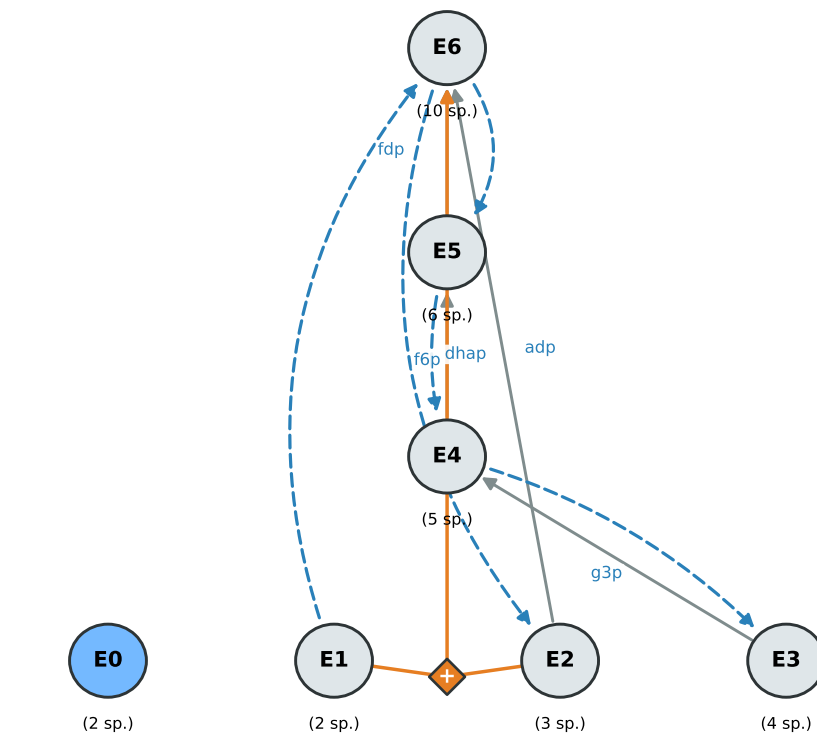
(b) Fundamental ERC hierarchy (containment, 1 synergy, complementarity chain)
