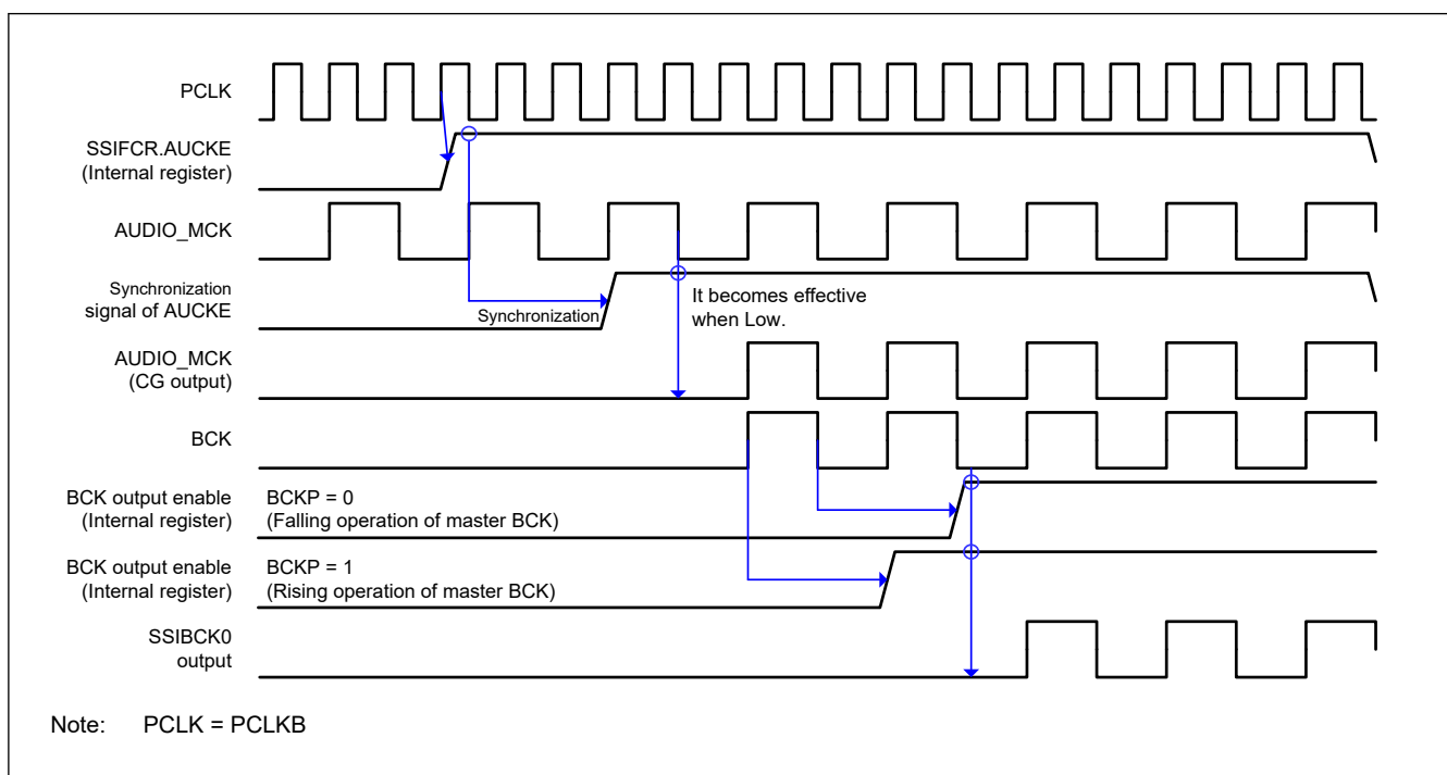
Figure 32.25 Timing diagram for the operation from system reset to start of master-mode communication
