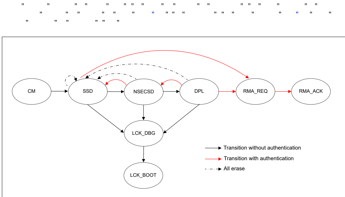
Figure 46.2 The illustration of the device lifecycle
