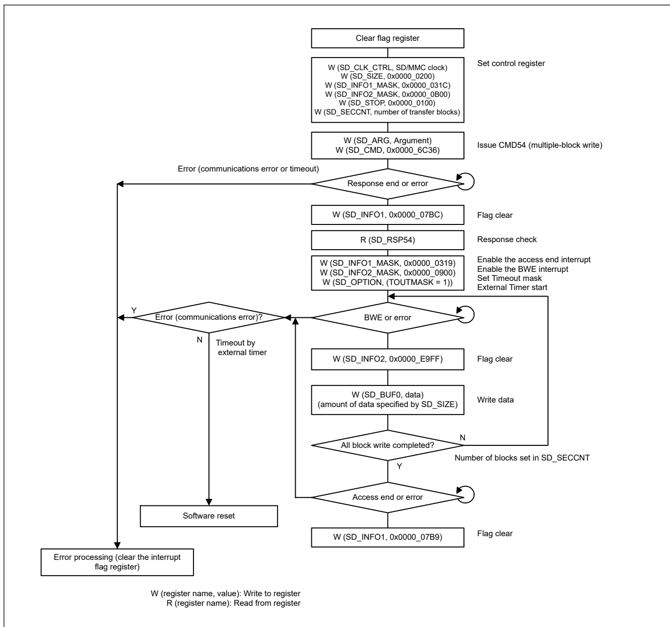
Figure 33.14 Example of multiple block write operation using external timer
