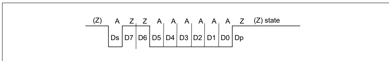
Figure 27.80 Inverse convention with SDIR in SCMR = 1, SINV in SCMR = 1, and PM in SMR_SMC1 = 1
