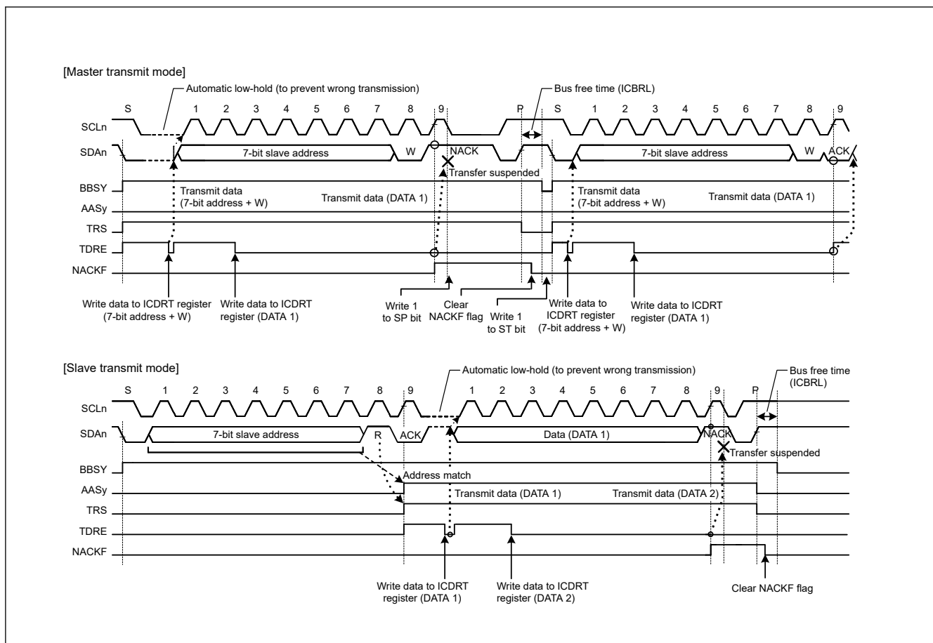
Figure 28.39 Suspension of data transfer when NACK is received, when NACKCE = 1
