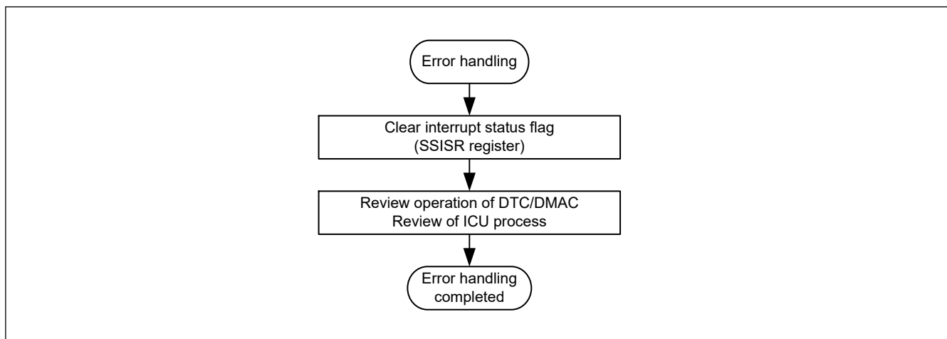
Figure 32.56 Error-handling procedure
