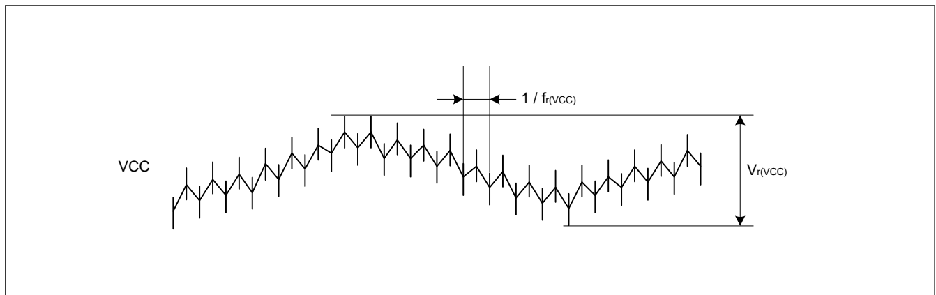
Figure 47.6 Ripple waveform
