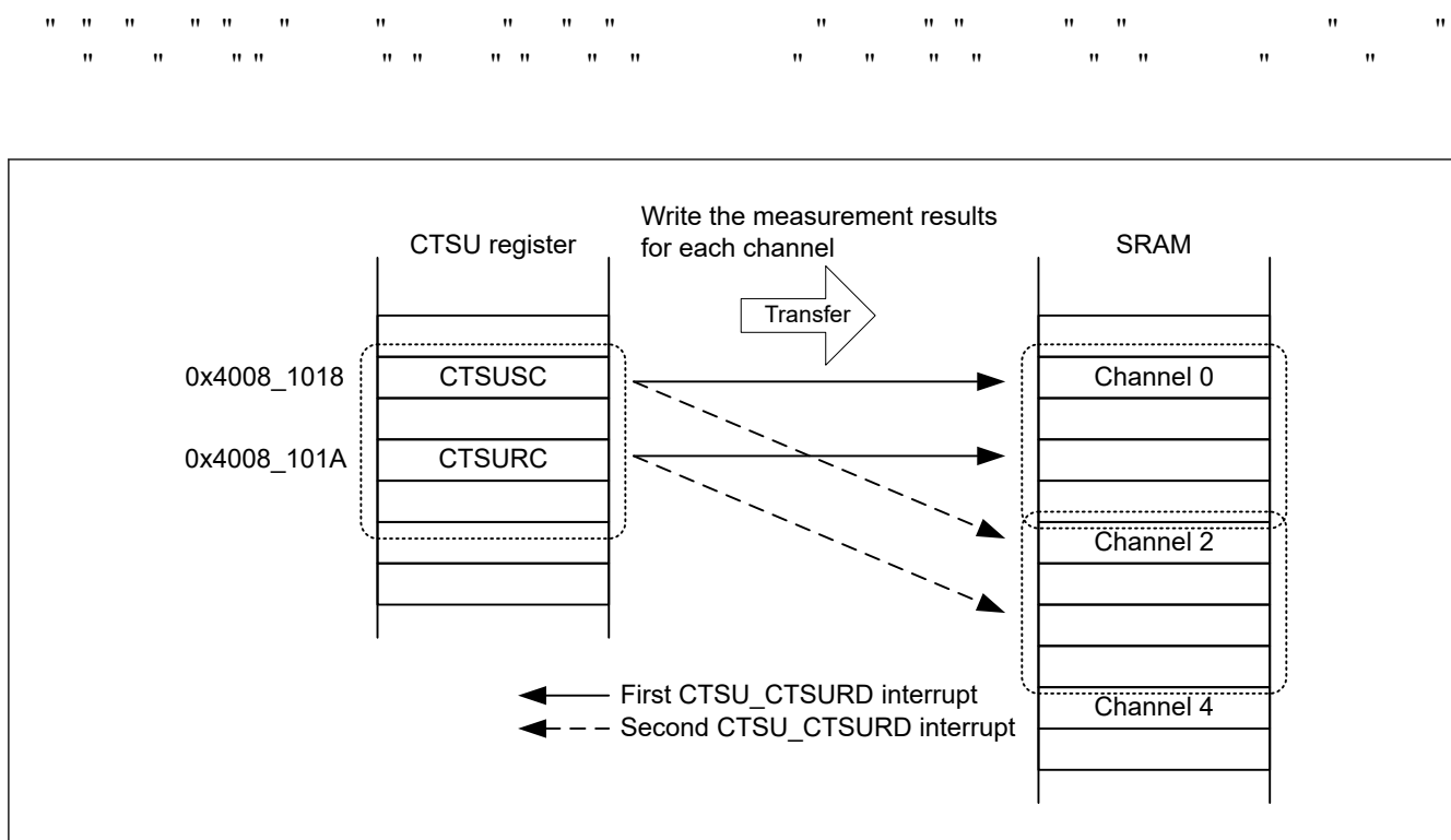
Figure 40.20 Example of DTC transfer operation using the CTSU_CTSURD interrupt
