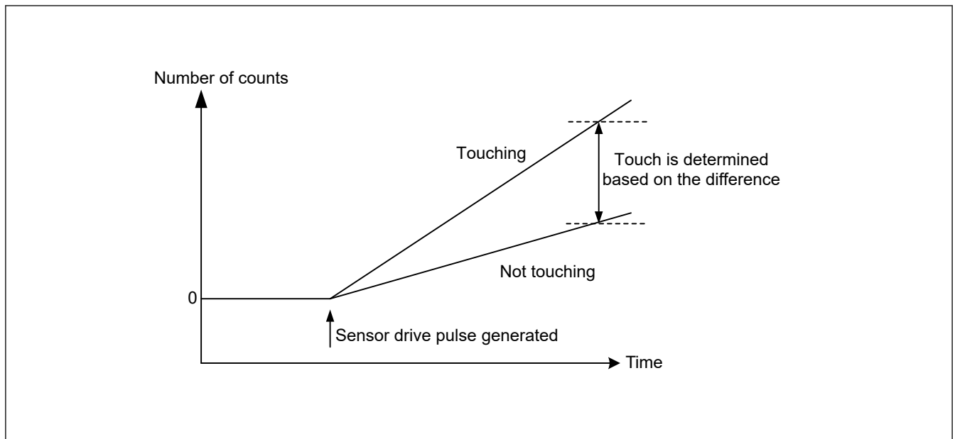
Figure 40.7 Change in measured value when finger is touching and not touching
