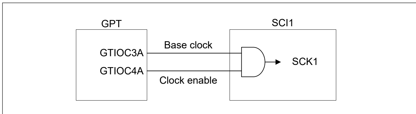
Figure 27.3 example of GPT and SCI connection
