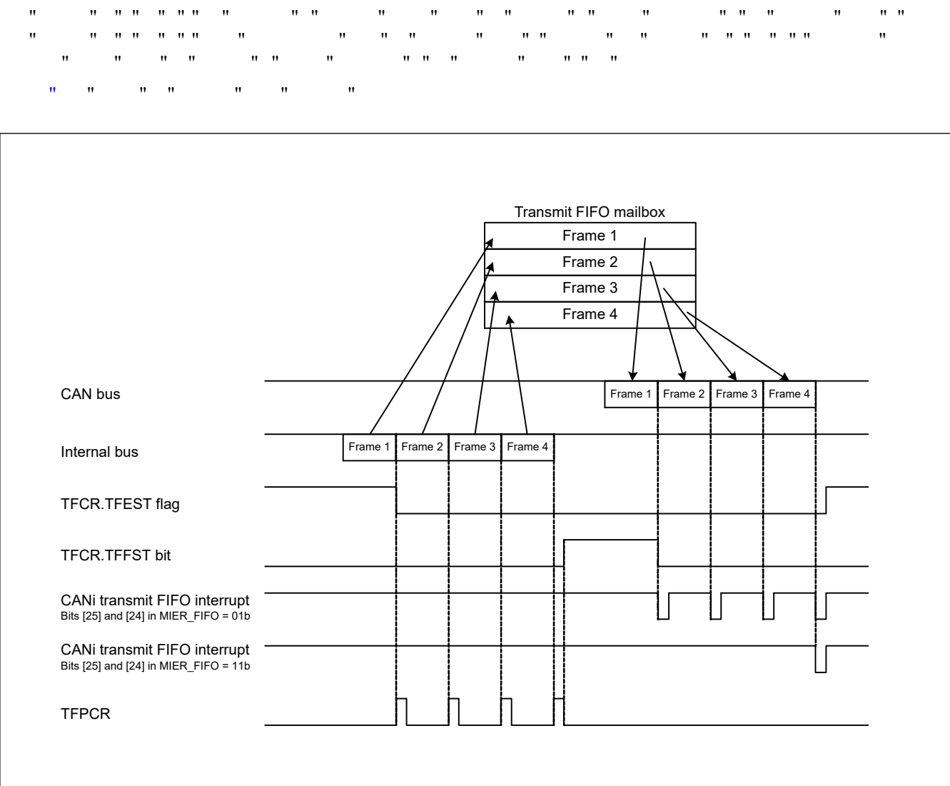
Figure 29.3 Transmit FIFO mailbox operation when bits [25] and [24] in MIER_FIFO = 01b or 11b
