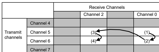
Figure 40.16 Software flow and example operation for mutual capacitance full scan mode
