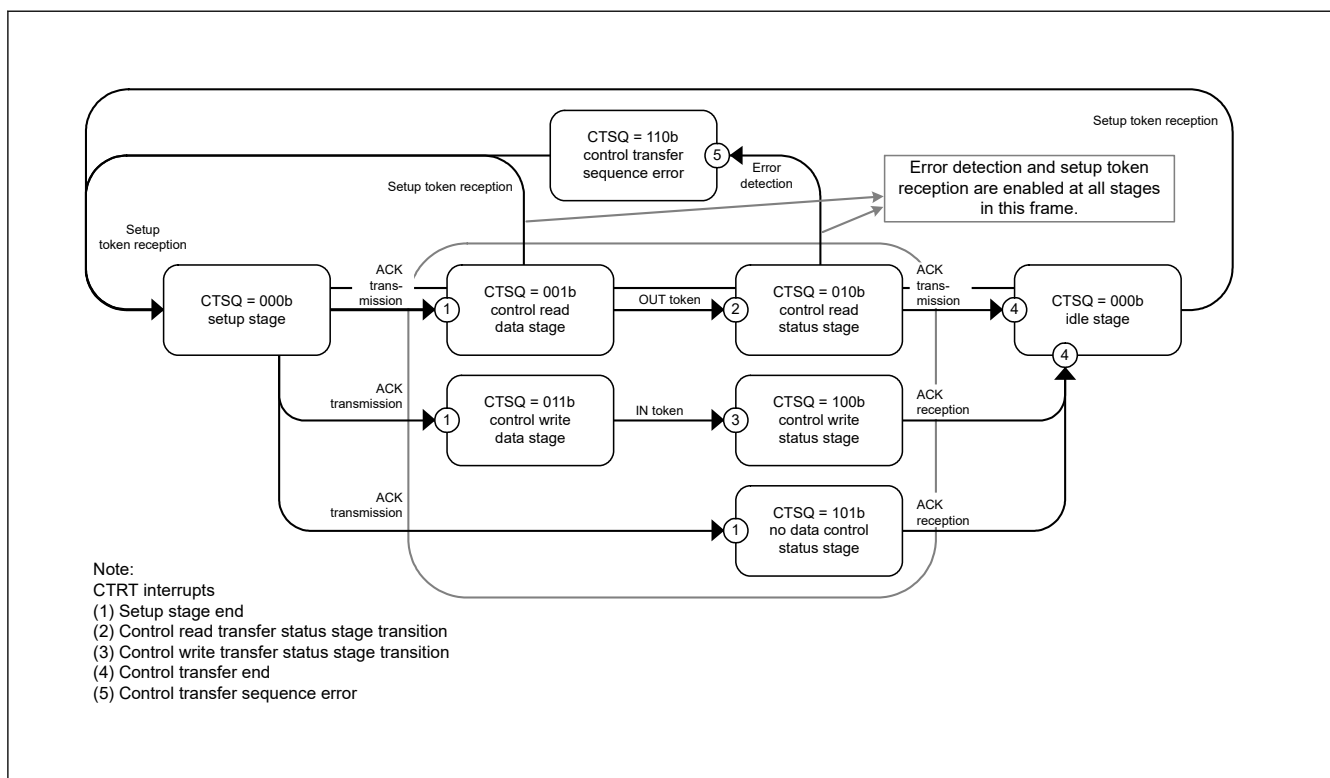
Figure 26.16 Control transfer stage transitions
