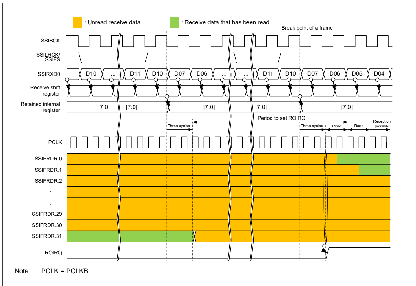
Figure 32.15 ROIRQ setting timing
