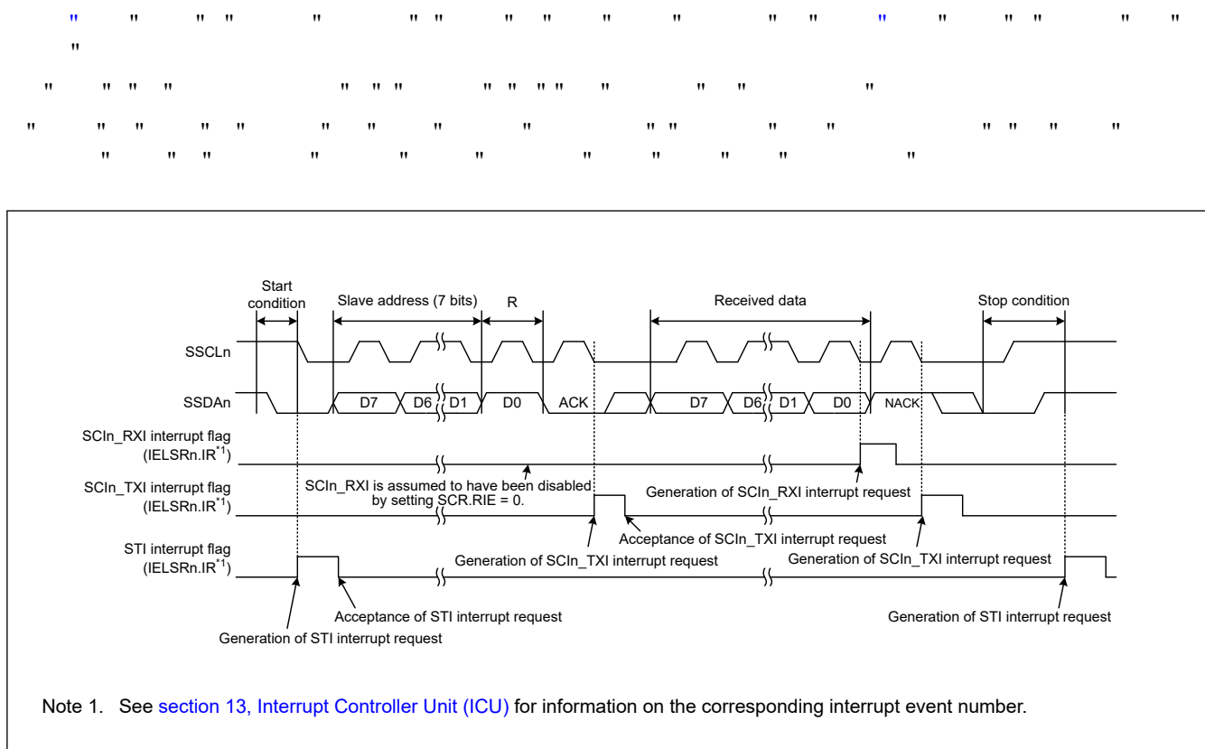
Figure 27.96 Example operations for master reception in simple IIC mode with 7-bit slave addresses, transmission interrupts, and reception interrupts
