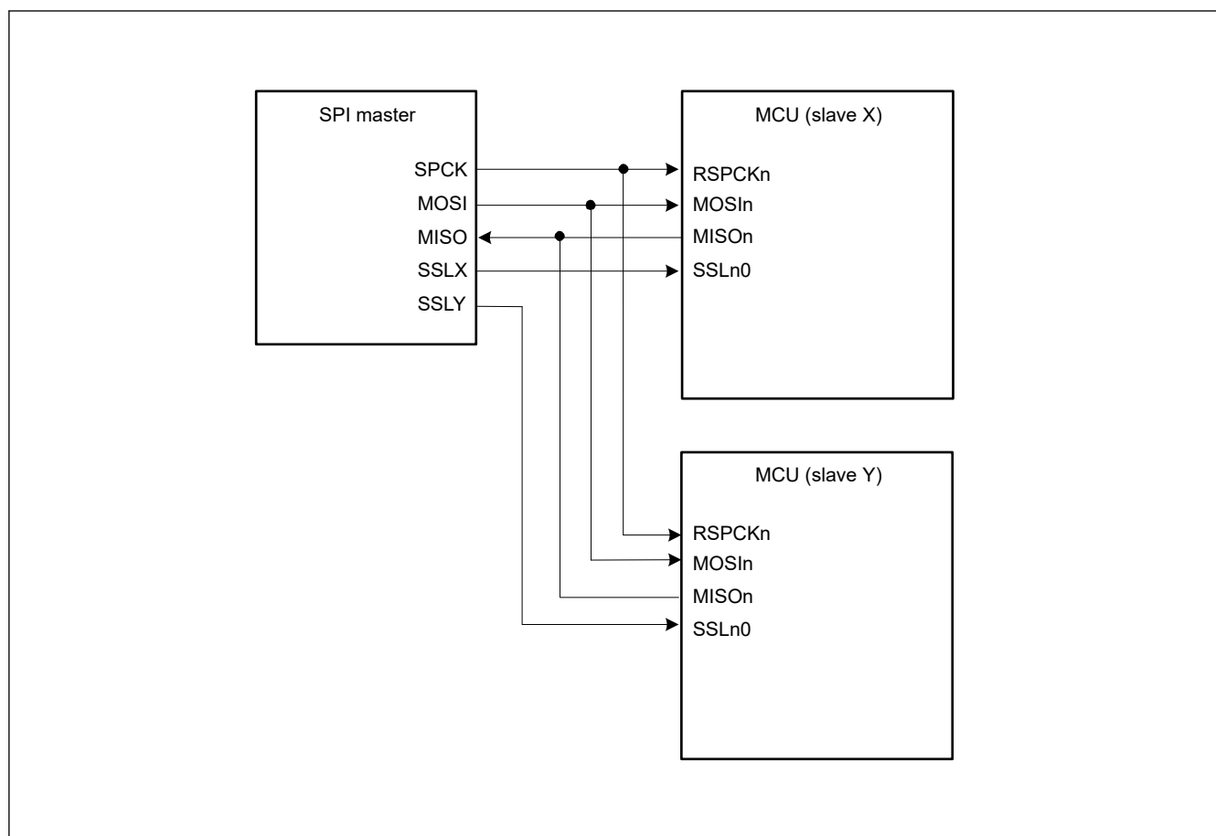
Figure 30.9 Single-master/multi-slave configuration example with the MCU as a slave
