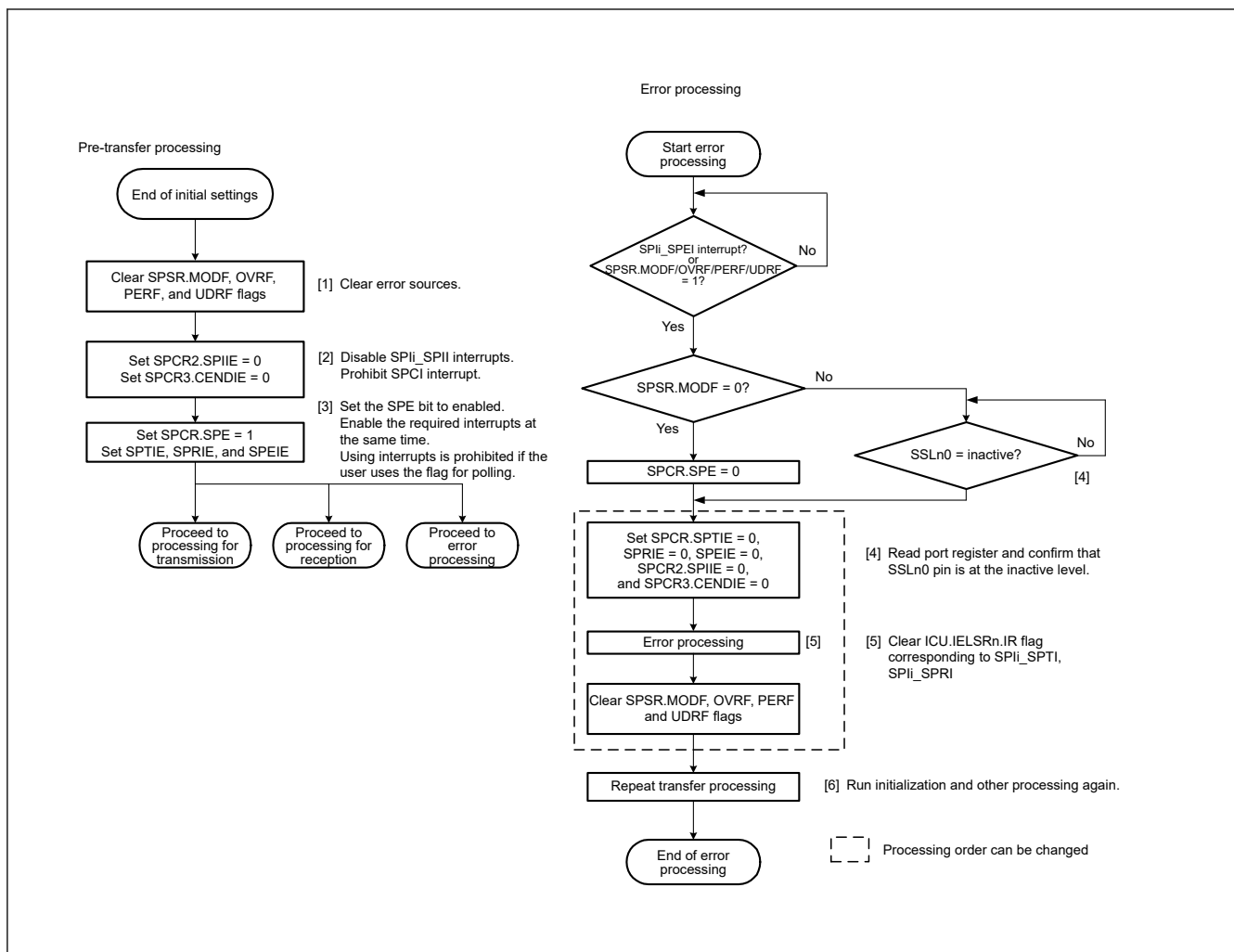
Figure 30.51 Error processing flow in master mode
