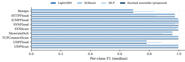
Fig. 3. Per-class F1 (median over ten seeds) on the cross-station split BS1 \rightarrow BS2. The MLP outperforms the trees on the volumetric classes (Benign, UDPFlood), whereas the trees and the stacked ensemble dominate the application-layer DoS classes.
