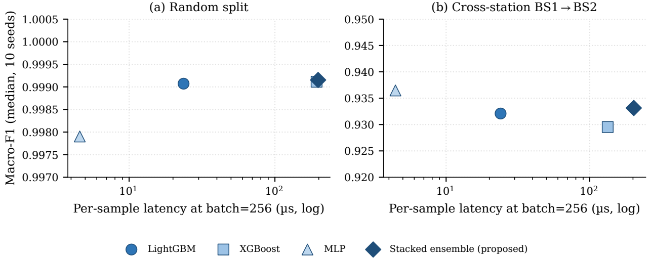
Fig. 1. Latency–accuracy Pareto operating points at batch size 256 on (a) the stratified random split and (b) the cross-station BS1 \rightarrow BS2 split. Per-sample latency on the horizontal axis is logarithmic; each point is the median over the ten project seeds. The random panel is near-saturated; the cross-station panel exposes the operational gap between MLP and the tree-based learners.
