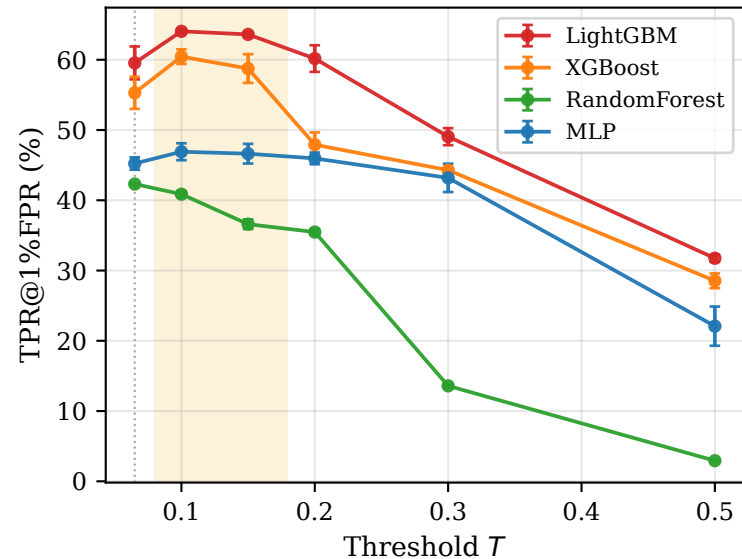
(a) Challenge TPR@1%FPR
