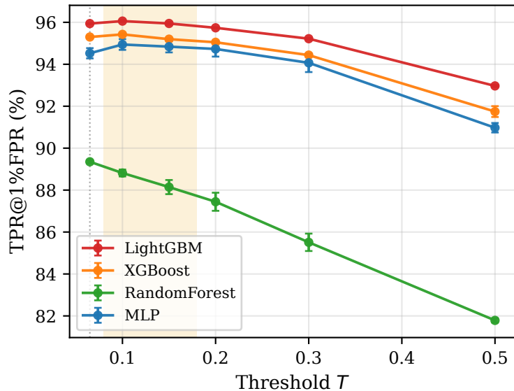
(b) Test TPR@1%FPR
