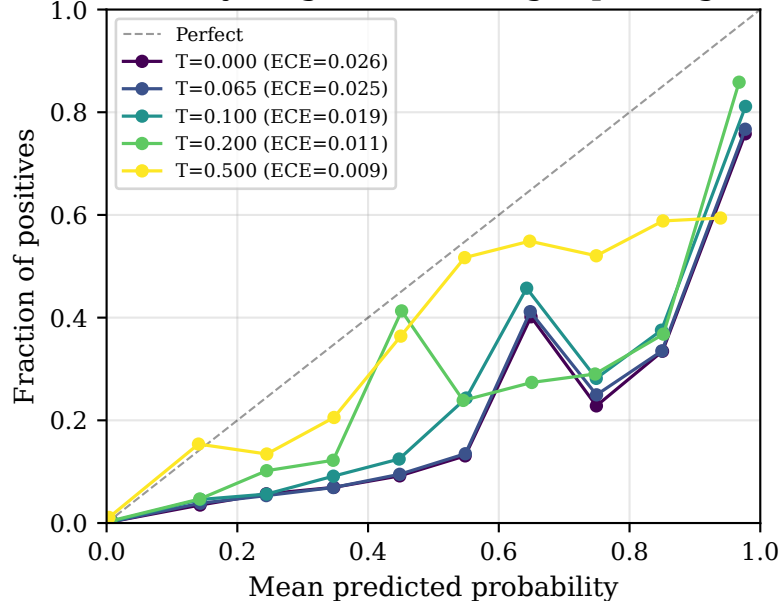
(a) Reliability diagram (challenge split, LightGBM) (b) Expected Calibration Error vs T (LightGBM)
