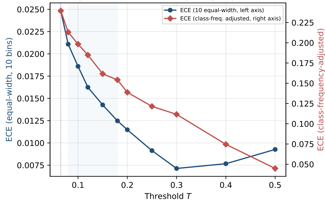
(a) Equal-width vs class-frequency-adjusted ECE
