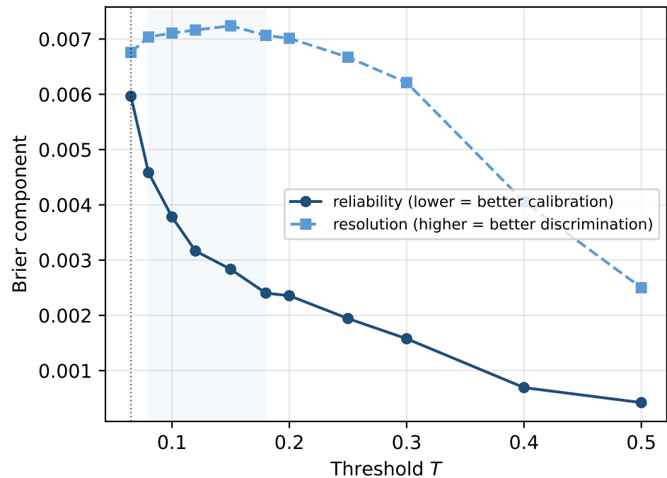
(b) Brier-decomposition components across T
