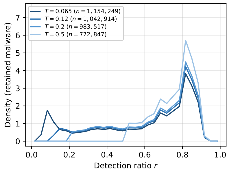
(c) Detection-ratio distribution shift
