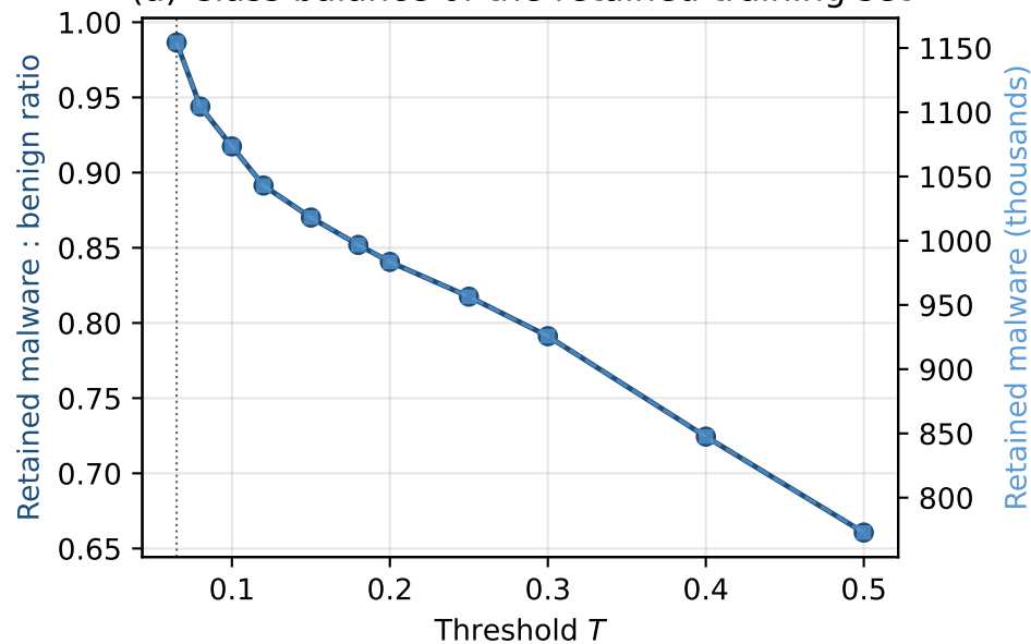
(a) Class balance of the retained training set
