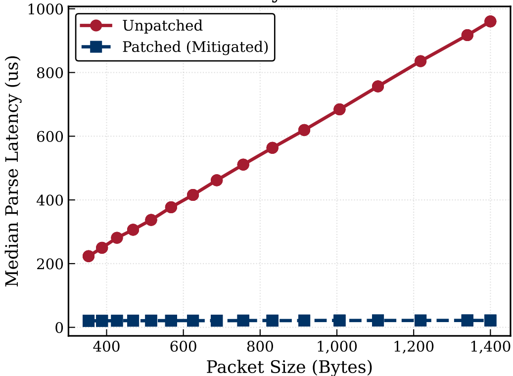
Parse Latency vs. Packet Size
