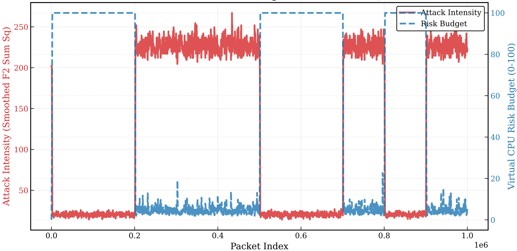
Attack Distribution vs Risk Budget Curve (Mode 3 @ 1.0%)
