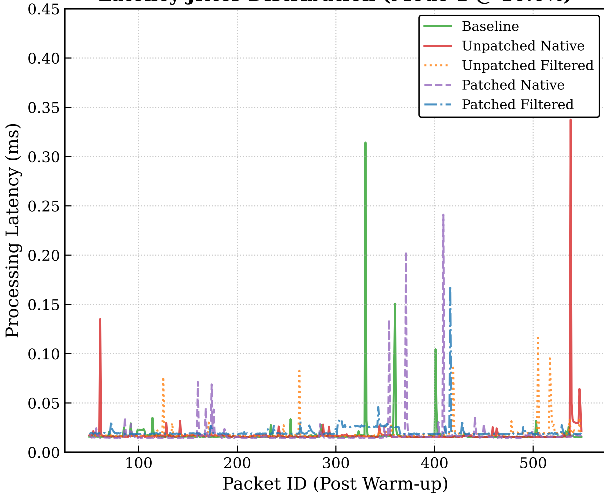
Latency Jitter Distribution (Mode 1 @ 10.0%)
