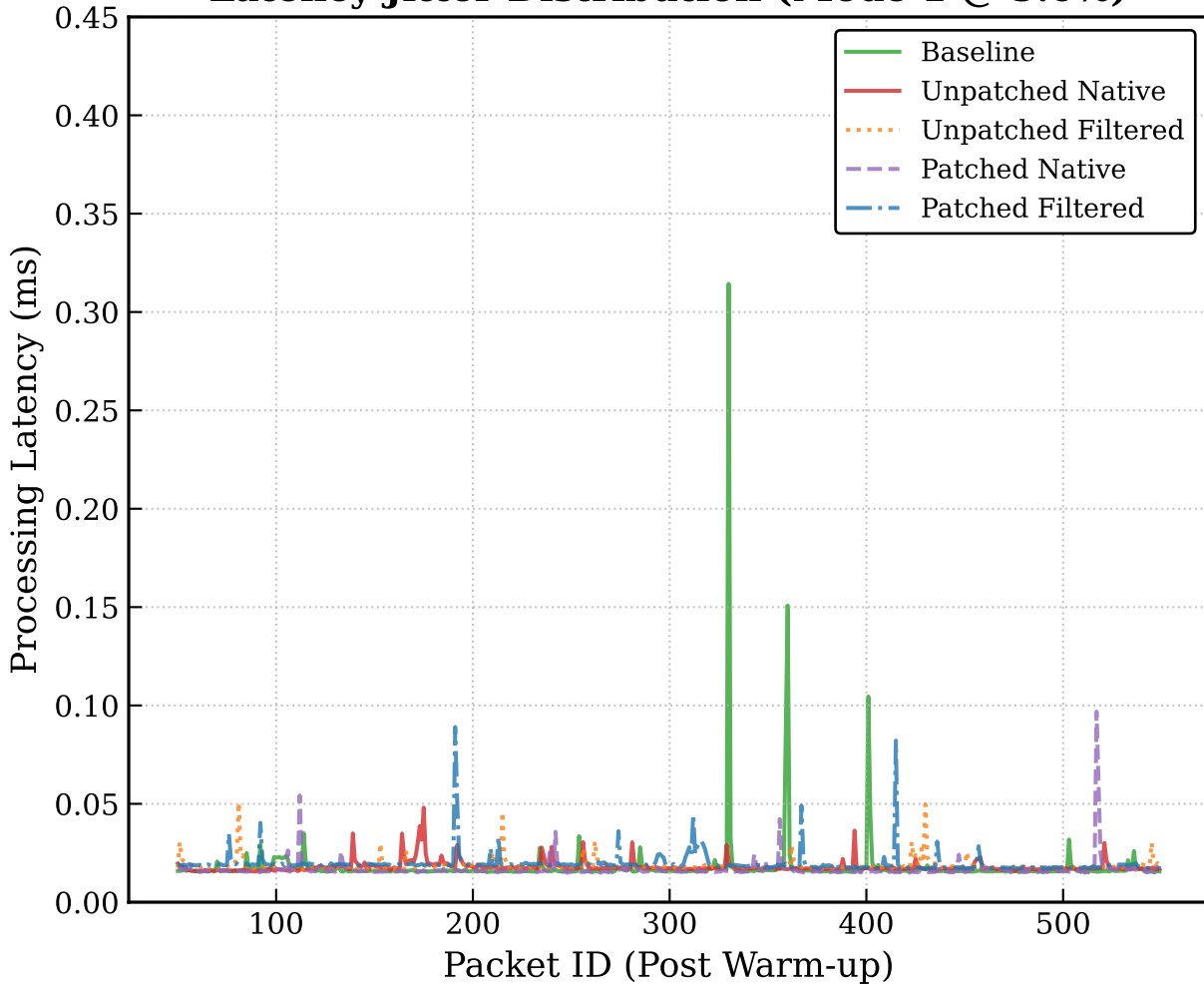
Latency Jitter Distribution (Mode 1 @ 5.0%)
