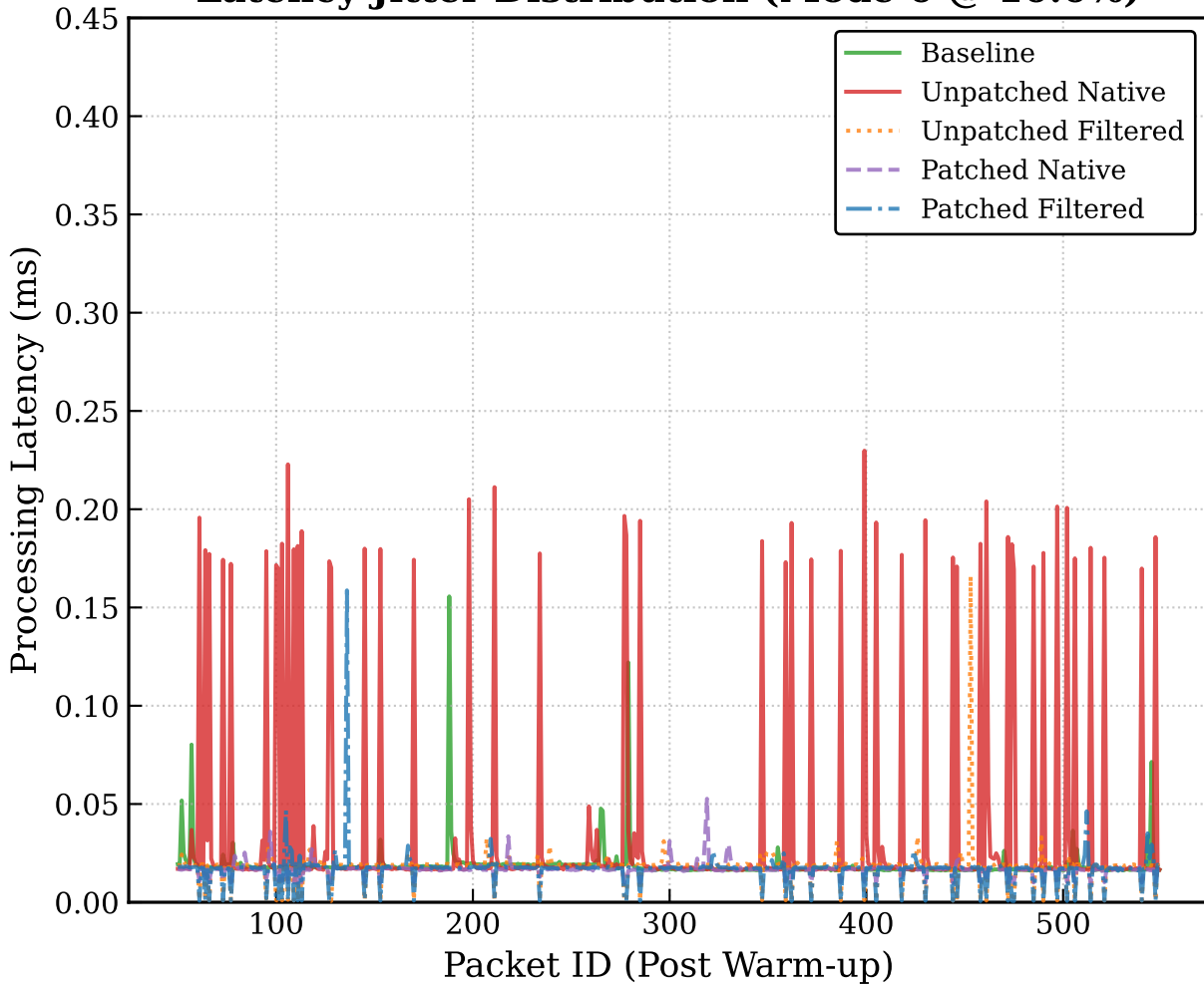
Latency Jitter Distribution (Mode 0 @ 10.0%)
