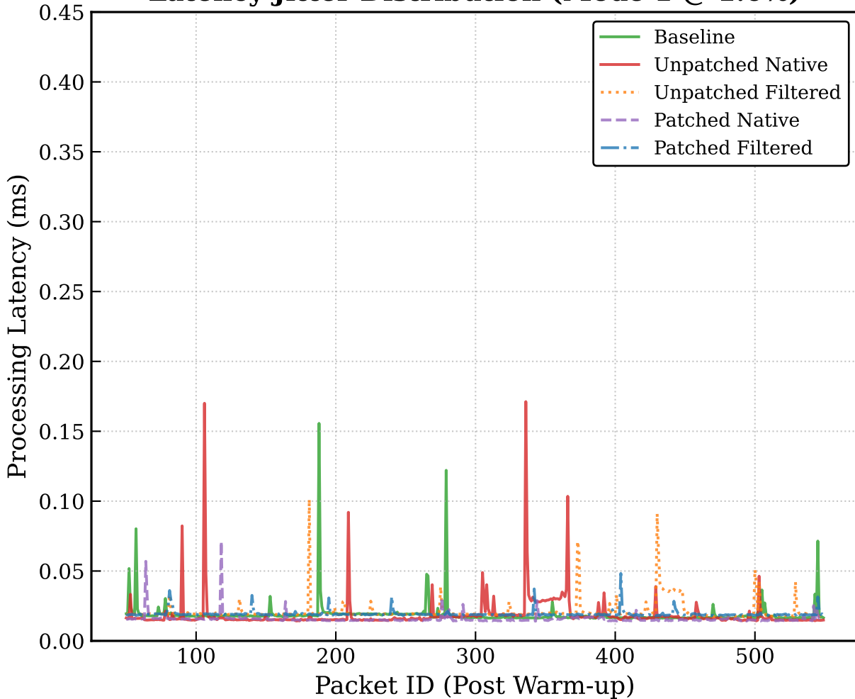
Latency Jitter Distribution (Mode 1 @ 1.0%)
