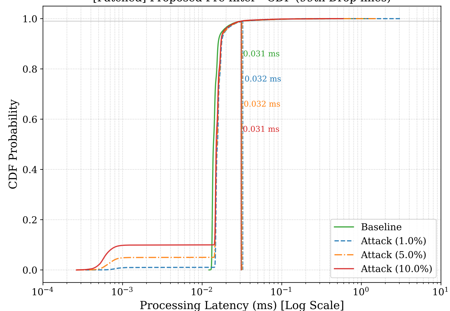
[Patched] Proposed Pre-filter - CDF (99th Drop-lines)
