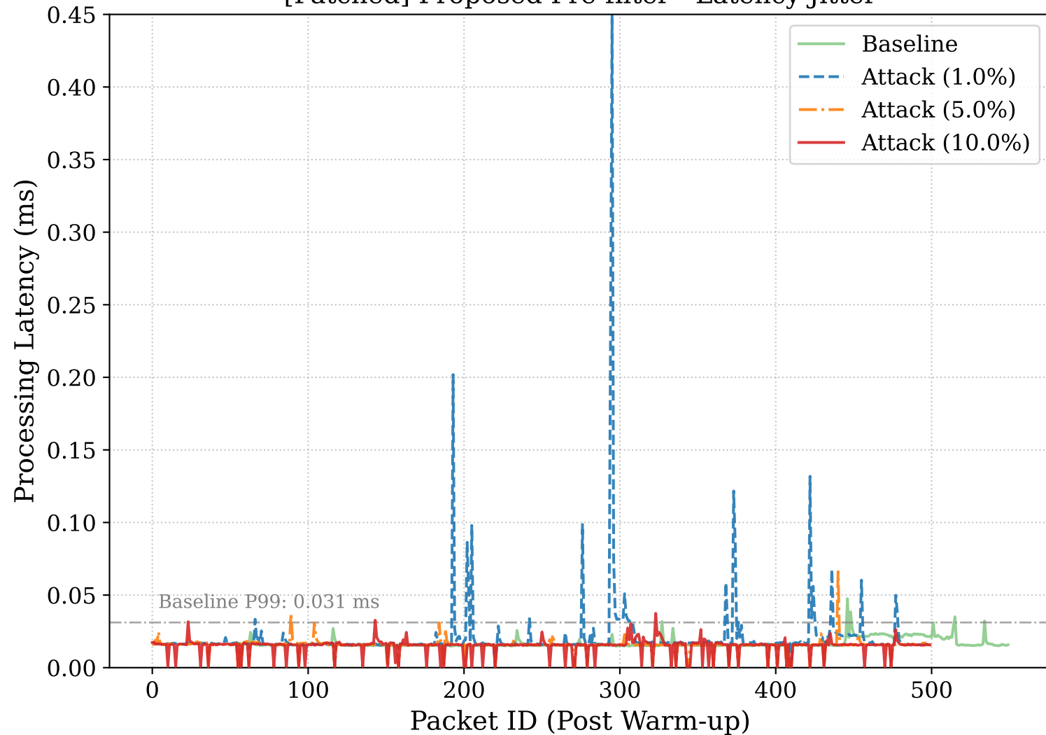
[Patched] Proposed Pre-filter - Latency Jitter
