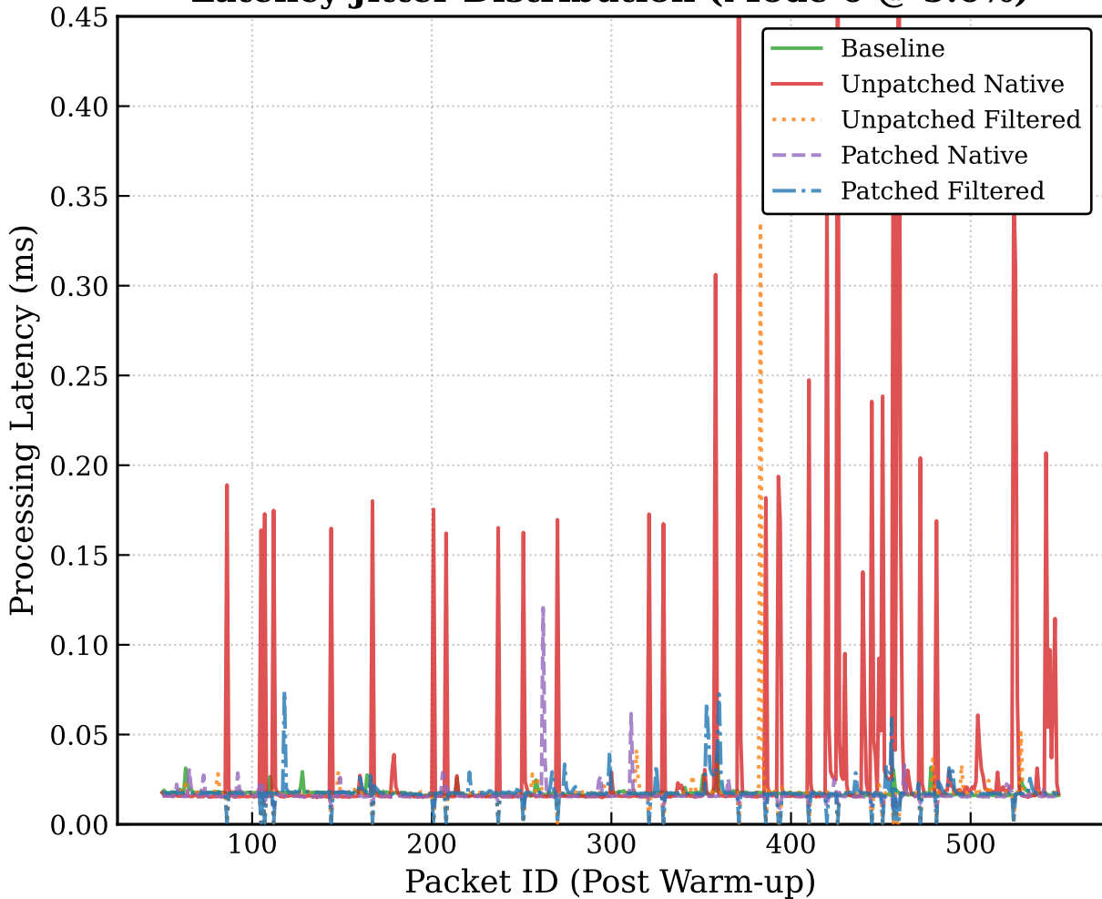
Latency Jitter Distribution (Mode 0 @ 5.0%)
