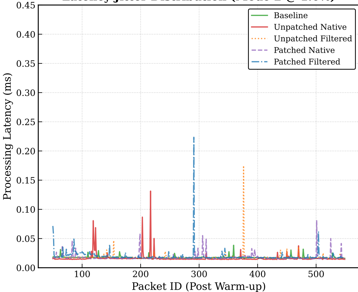
Latency Jitter Distribution (Mode 2 @ 1.0%)
