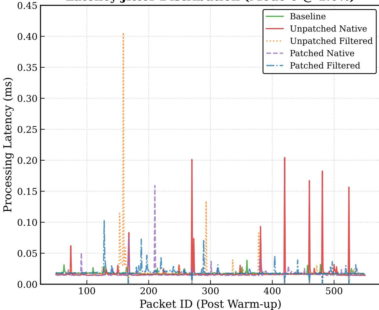
Latency Jitter Distribution (Mode 0 @ 1.0%)
