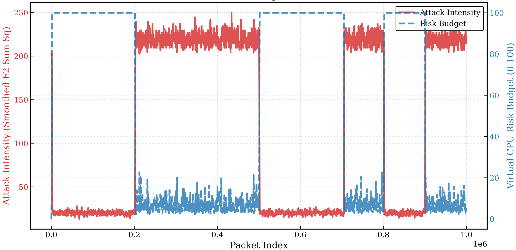
Attack Distribution vs Risk Budget Curve (Mode 3 @ 0.7%)
