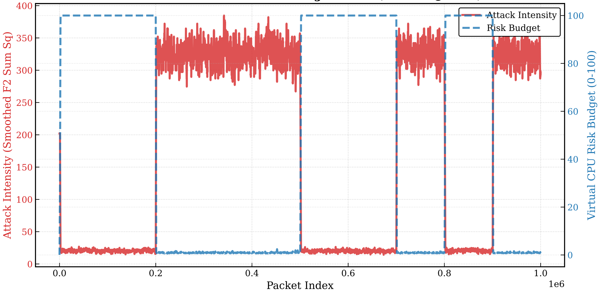
Attack Distribution vs Risk Budget Curve (Mode 3 @ 5.0%)
