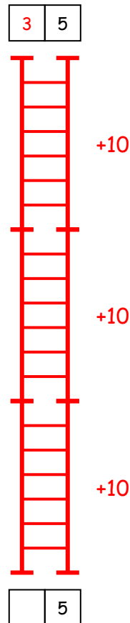
Figure 3.21: Climbing three ladders means adding 3 \times 10 = 10 + 10 + 10 = 30 .
