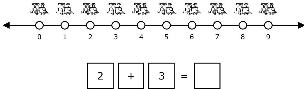
Figure 2.10: Compute 2 + 3 on the number line.
