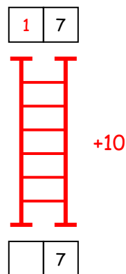
Figure 3.14: Climbing a ladder means adding 10.
