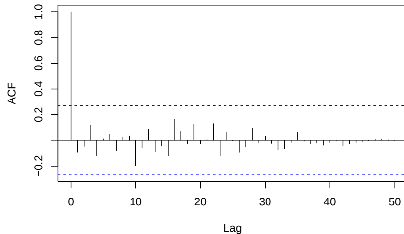
ACF of Residuals for ARIMA(13,1,1) for TLB with log transformation
