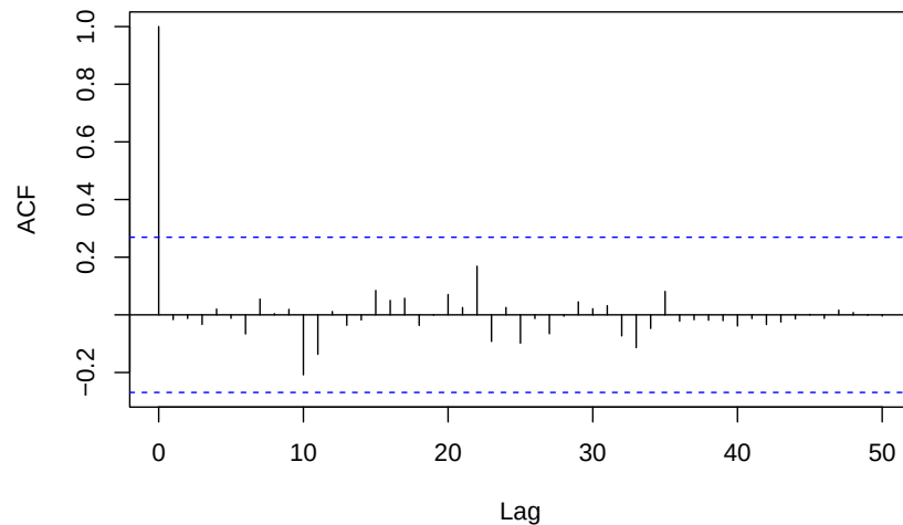
ACF of Residuals for ARIMA(15,1,1) for TLB with log transformation
