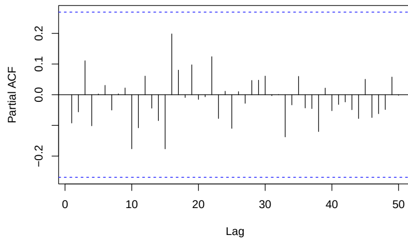
PACF of Residuals for ARIMA(13,1,1) for TLB with log transformation
