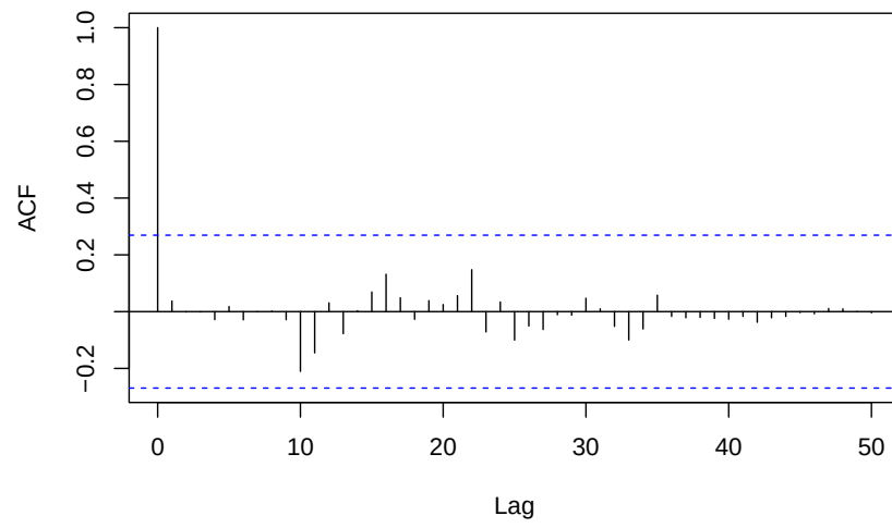
ACF of Residuals for ARIMA(15,1,0) for TLB with log transformation
