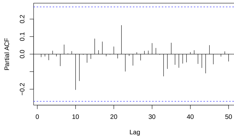
PACF of Residuals for ARIMA(15,1,1) for TLB with log transformation
