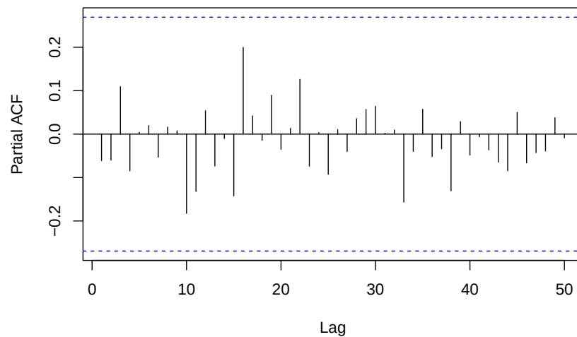
PACF of Residuals for ARIMA(14,1,1) for TLB with log transformation
