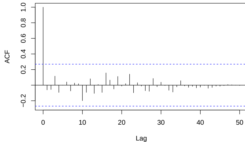
ACF of Residuals for ARIMA(14,1,1) for TLB with log transformation
