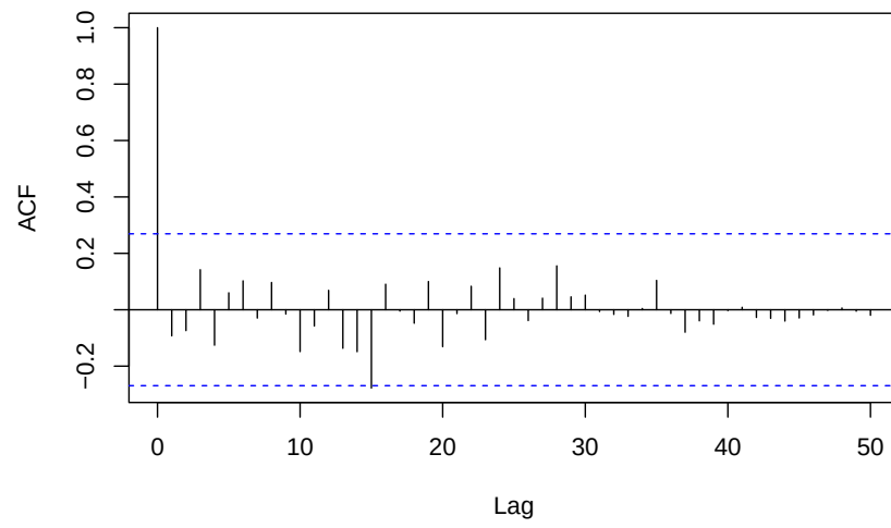
ACF of Residuals for ARIMA(13,1,0) for TFR with log transformation
