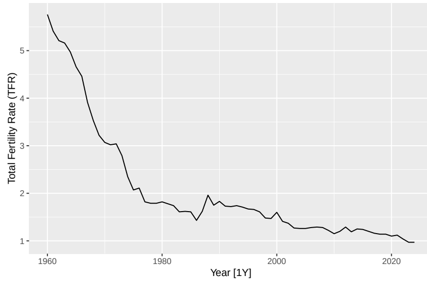
Figure 1. Initial Plot of Total Fertility Rate (TFR)
