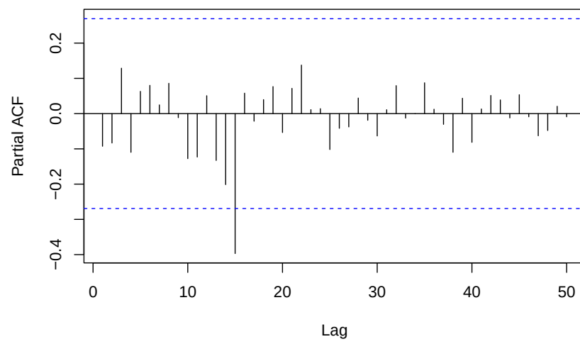
PACF of Residuals for ARIMA(13,1,0) for TFR with log transformation
