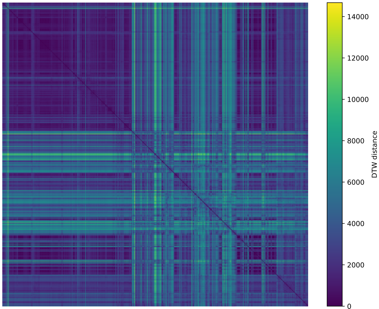
DTW distance matrix
