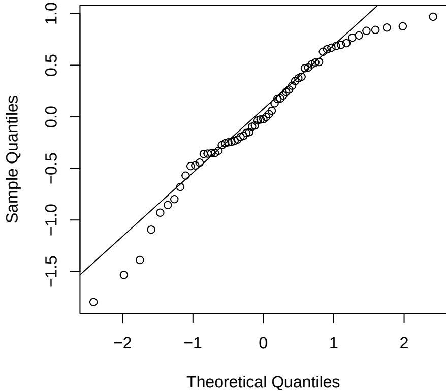
Random Intercepts
