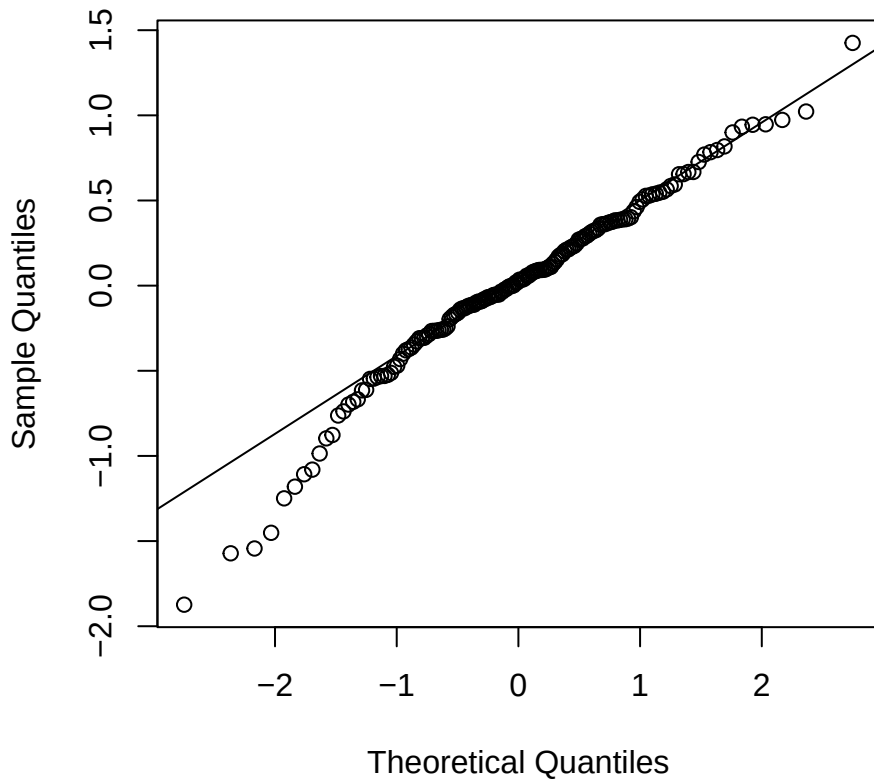
Random Intercepts
