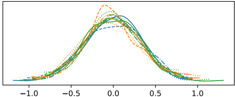
mu_model
