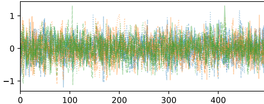
mu_model
