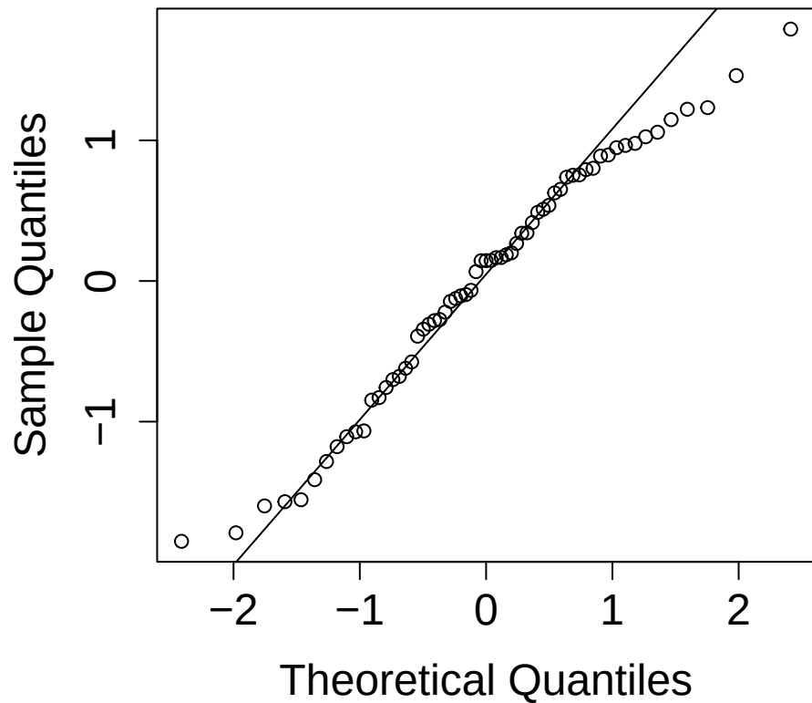
Random Intercepts
