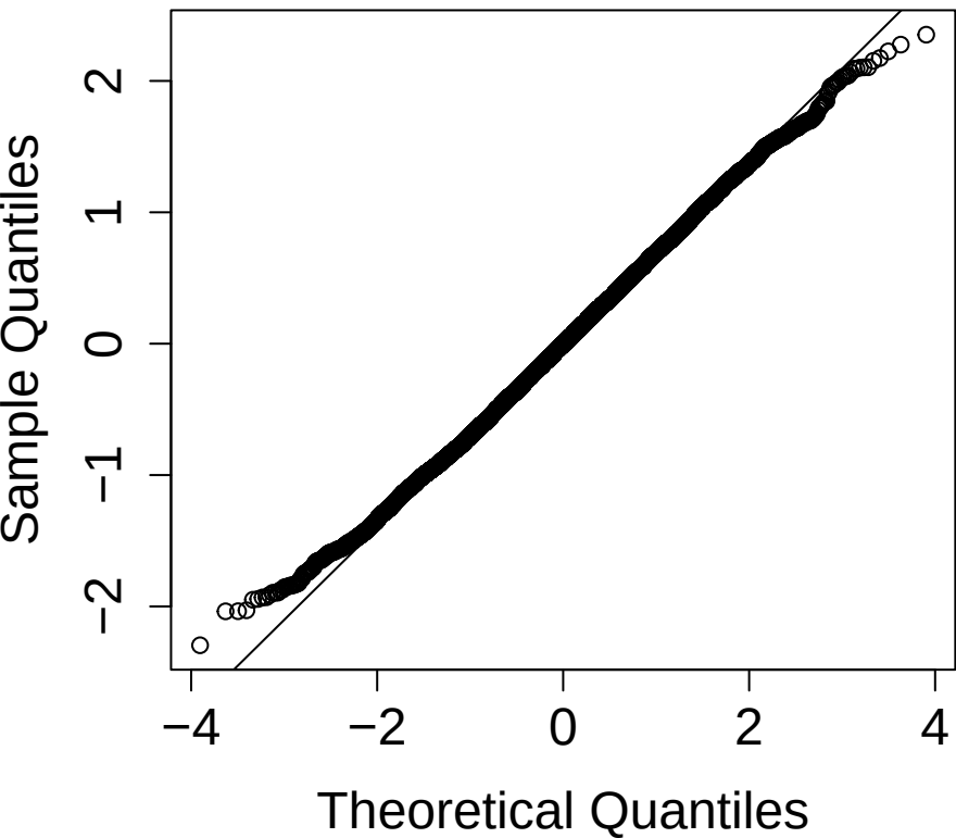
Residuals
