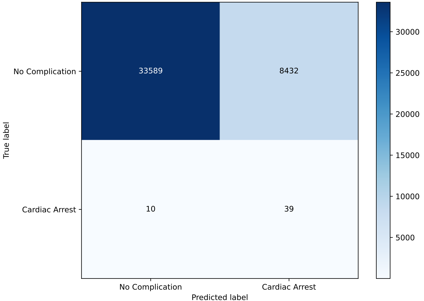
Confusion Matrix - CDARREST - Best Recall Model: 2layer_cnn (Recall = 0.7959)
