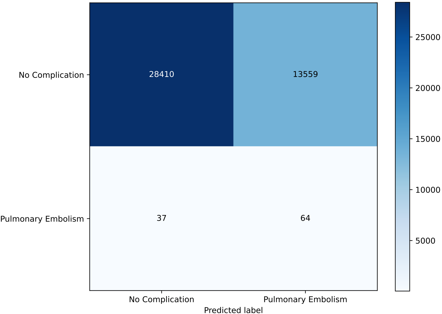
Confusion Matrix - PULEMBOL - Best Recall Model: lr (Recall = 0.6337)
