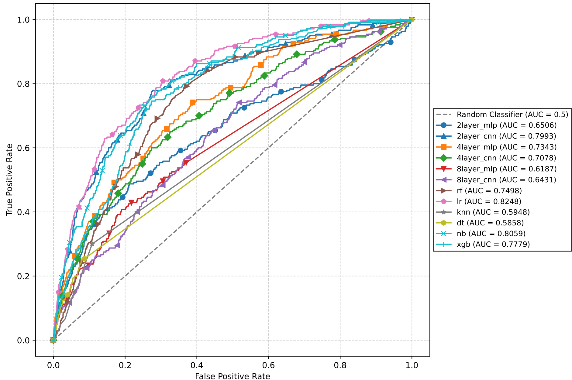
ROC Curve - OUPNEUMO (Best Models)
