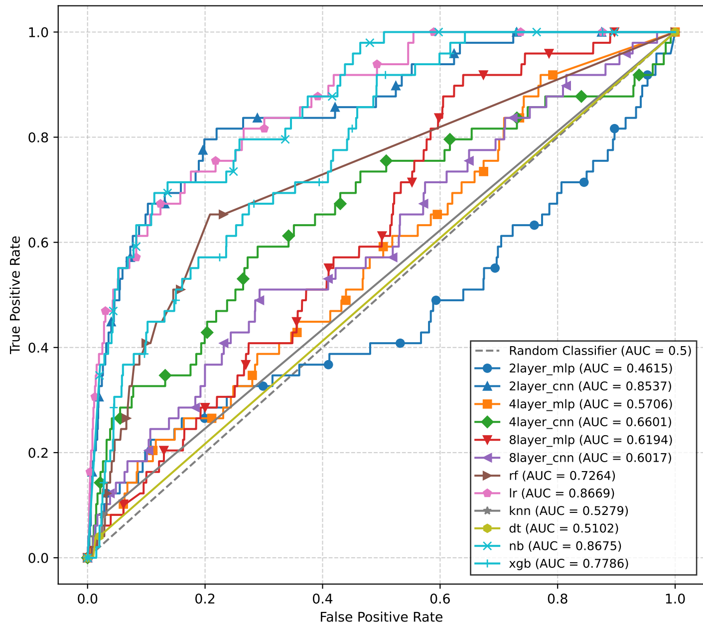
ROC Curve - CDARREST (Best Models)
