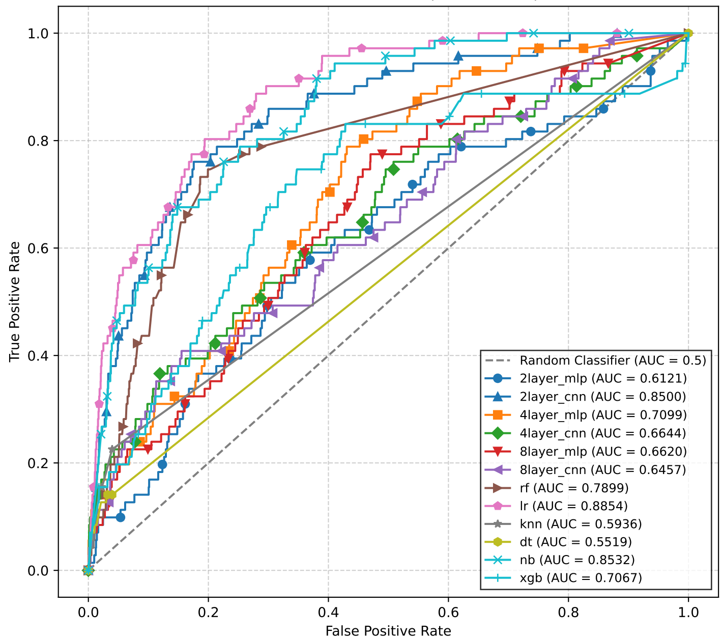
ROC Curve - FAILWEAN (Best Models)
