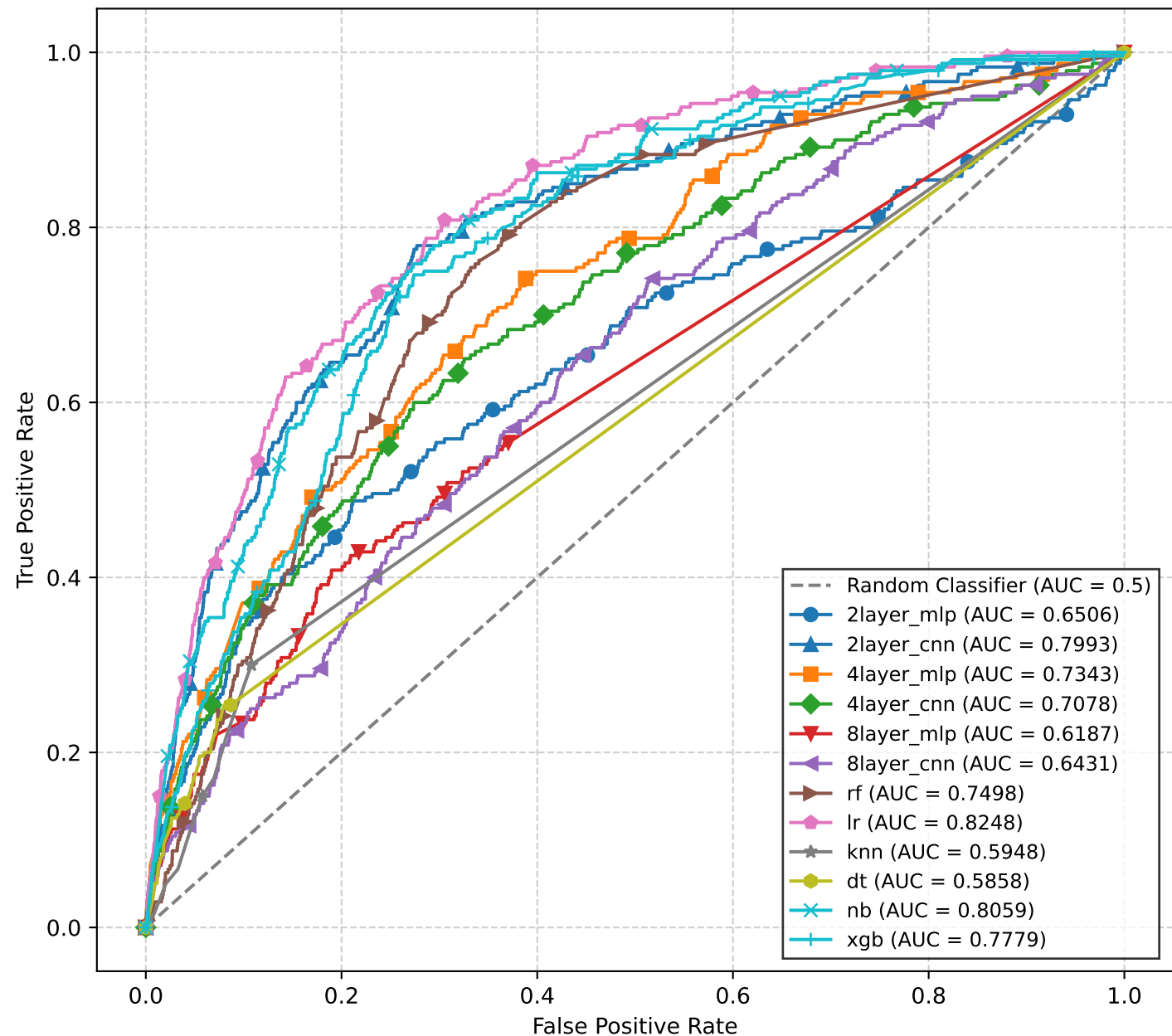
ROC Curve - OUPNEUMO (Best Models)
