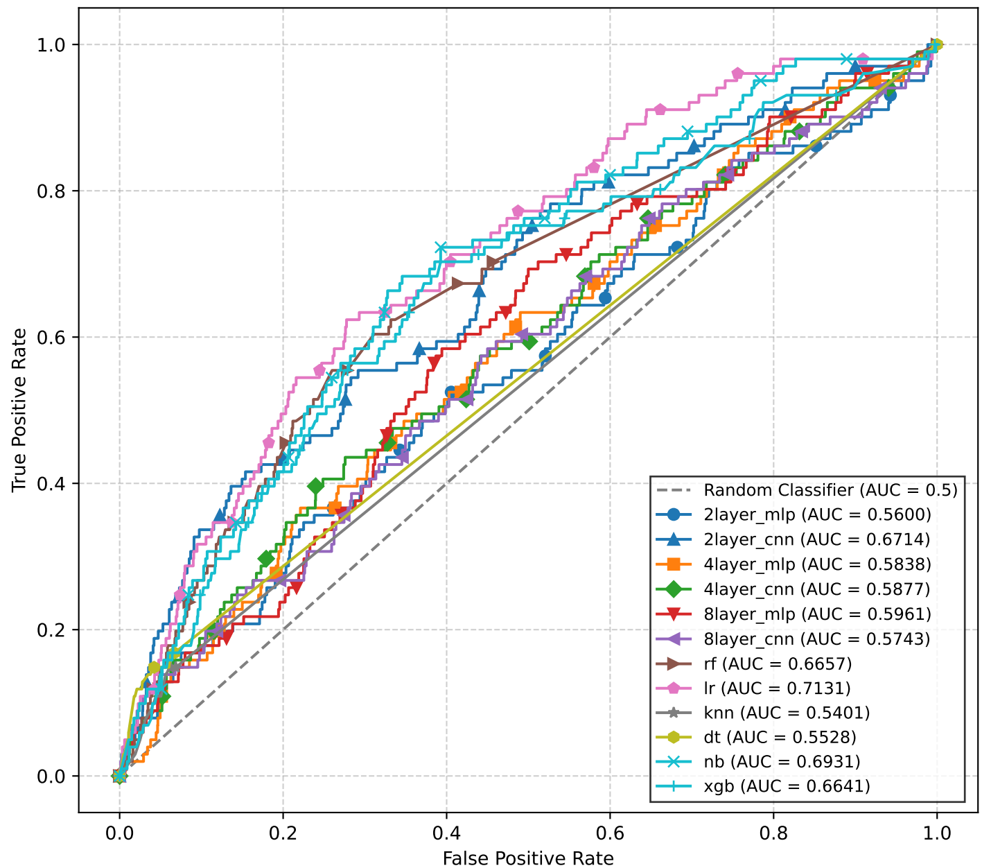
ROC Curve - PULEMBOL (Best Models)
