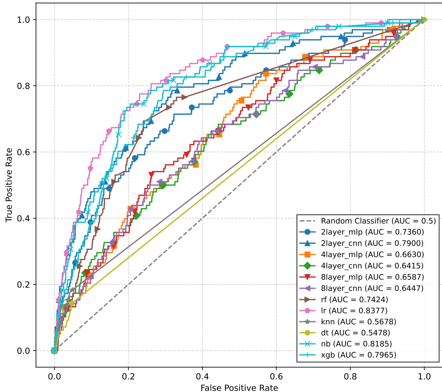
ROC Curve - REINTUB (Best Models)
