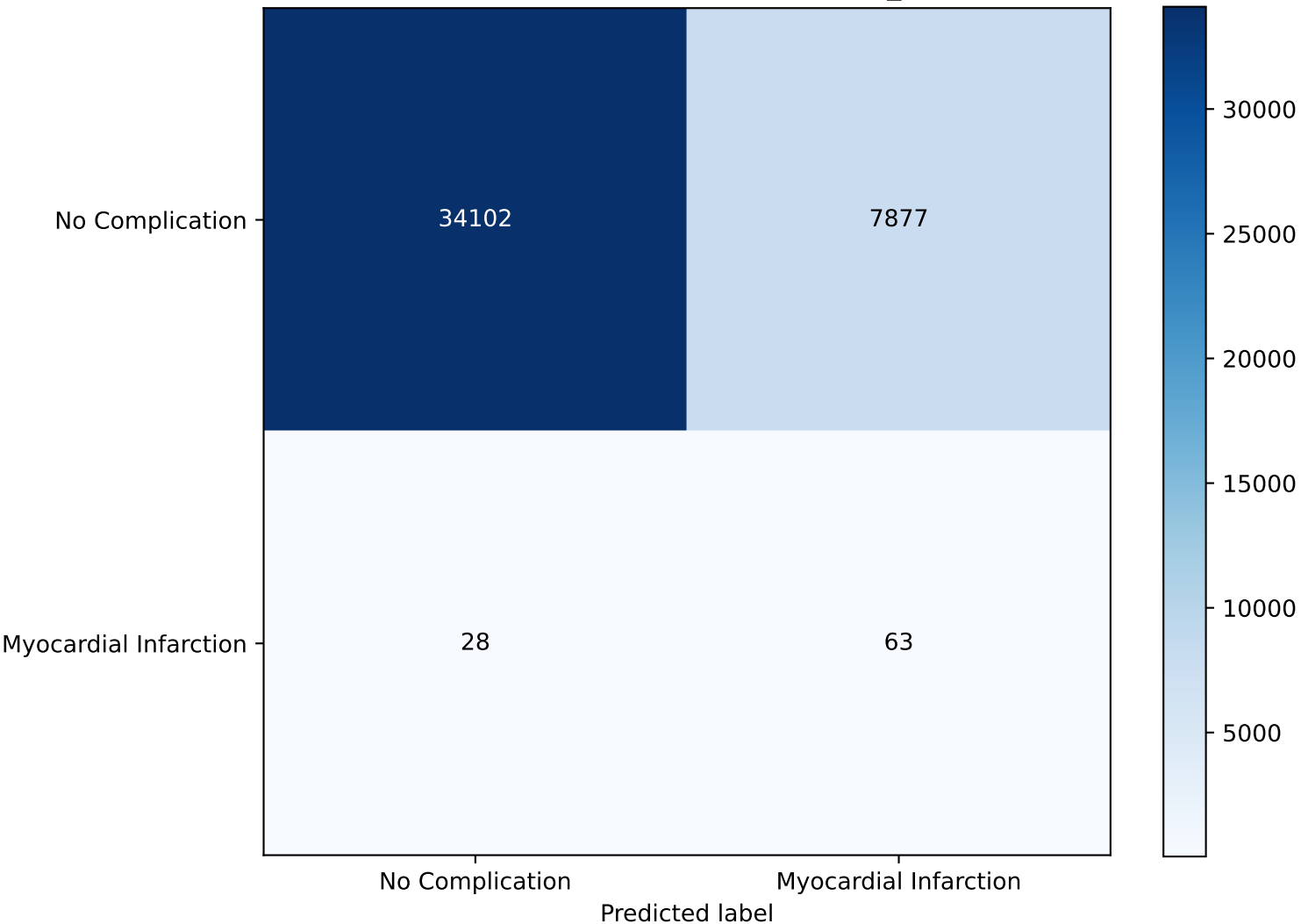
Confusion Matrix - CDMI - Best AUC Model: 4layer_mlp (AUC = 0.8428)
