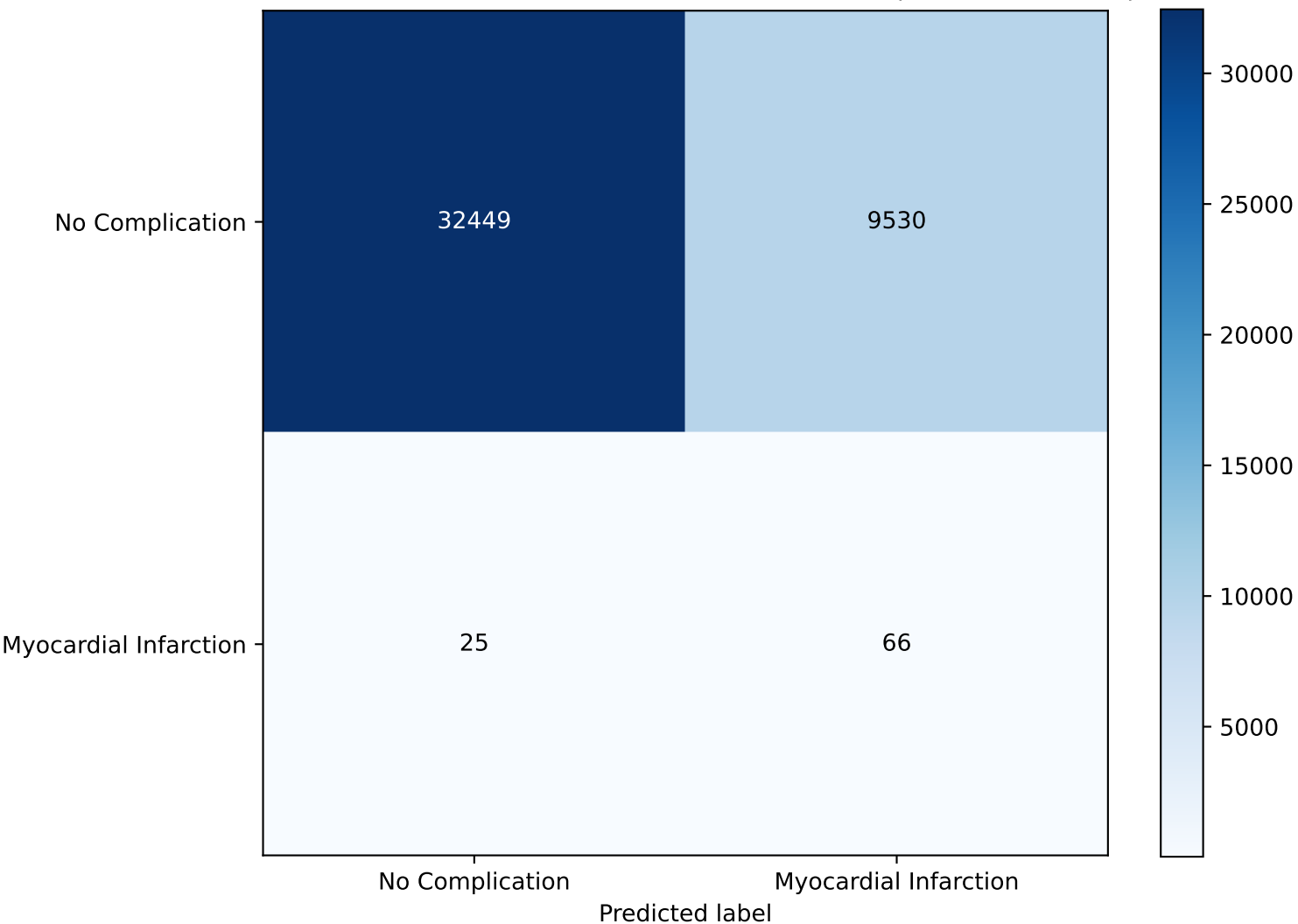
Confusion Matrix - CDMI - Best Recall Model: Ir (Recall = 0.7253)
