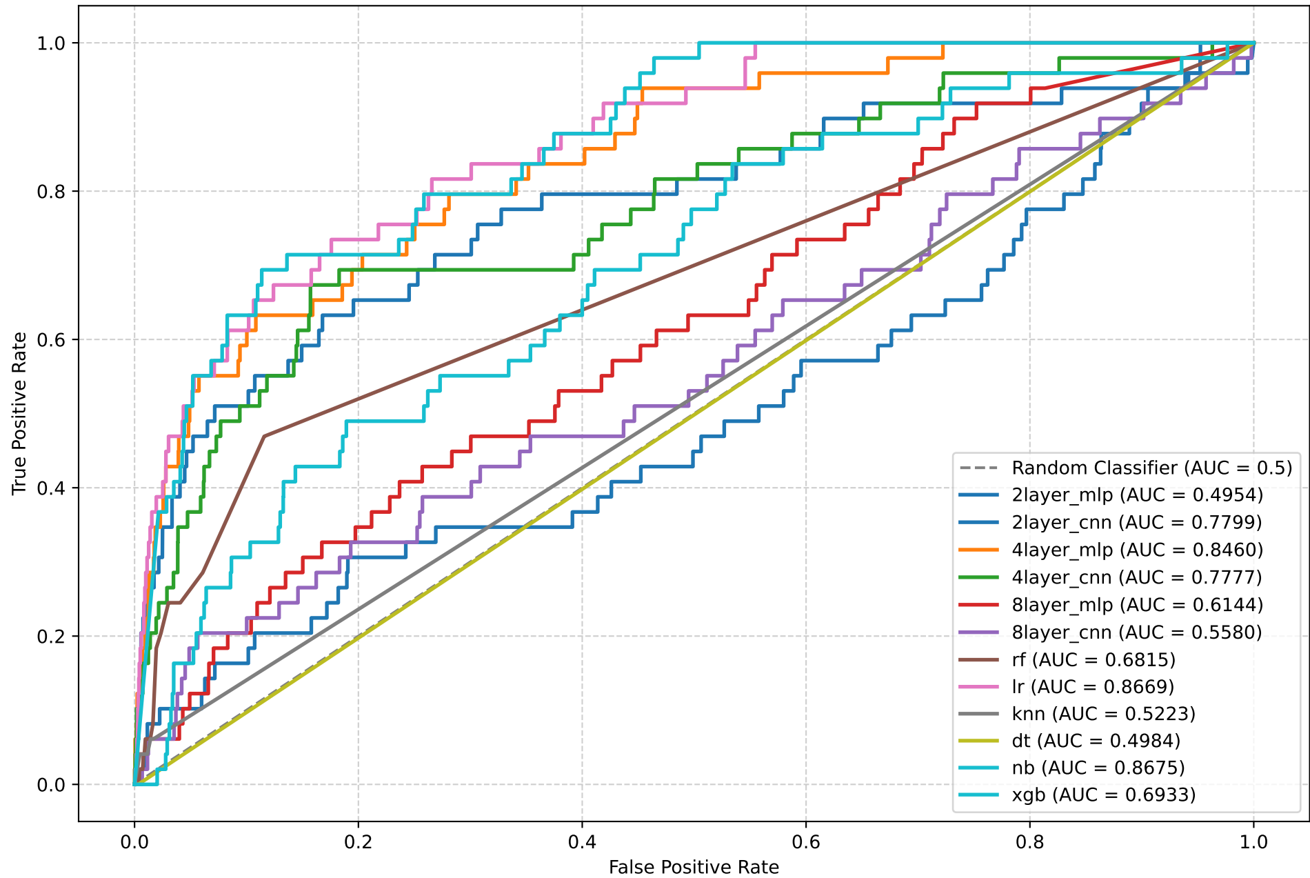
ROC Curve - CDARREST
