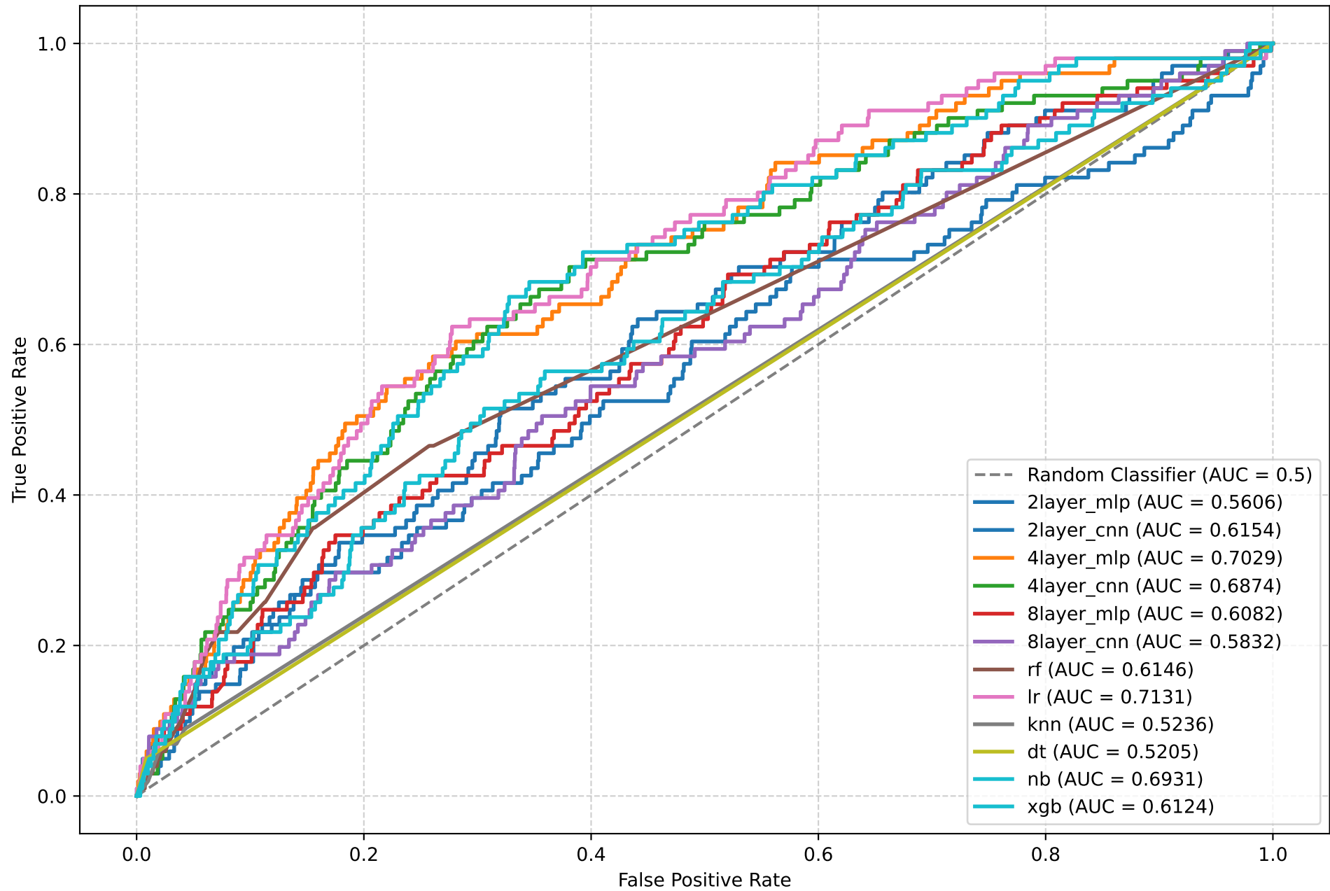
ROC Curve - PULEMBOL
