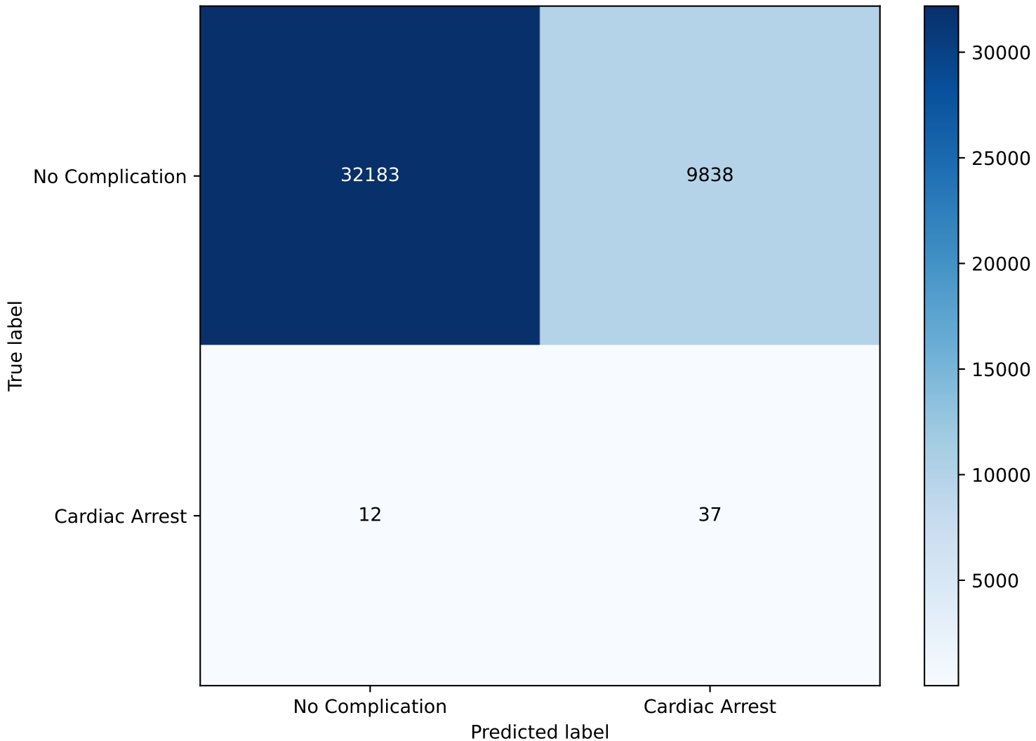
Confusion Matrix - CDARREST - Best Recall Model: lr (Recall = 0.7551)
