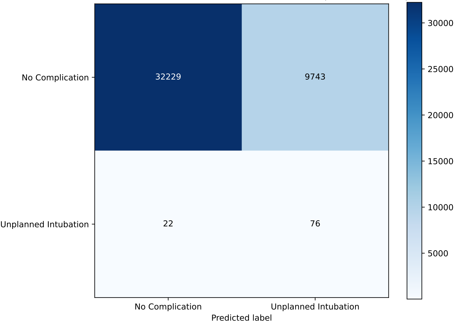
Confusion Matrix - REINTUB - Best Recall Model: Ir (Recall = 0.7755)
